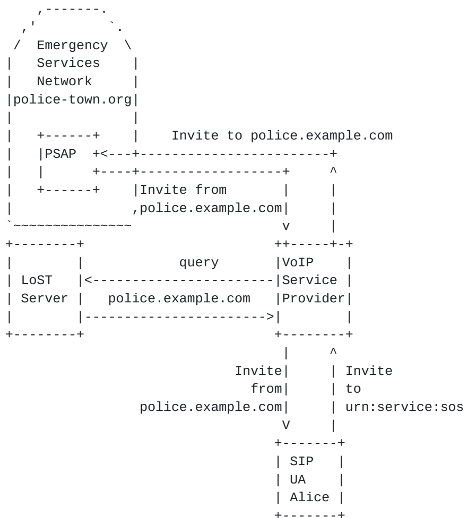
Figure 4: Example for Network-based Service URN Resolution.
