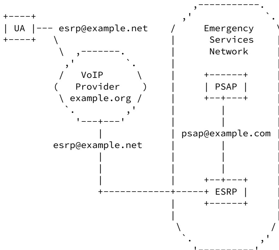
Figure 2: Example for Multi-Stage Routing.
