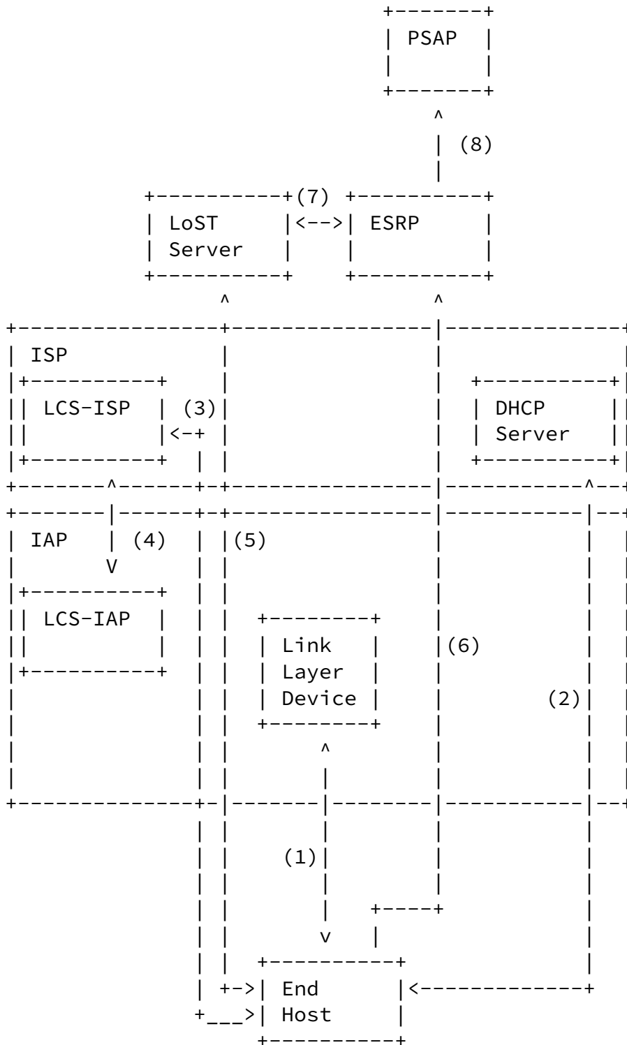
Figure 2: Architectural Overview
