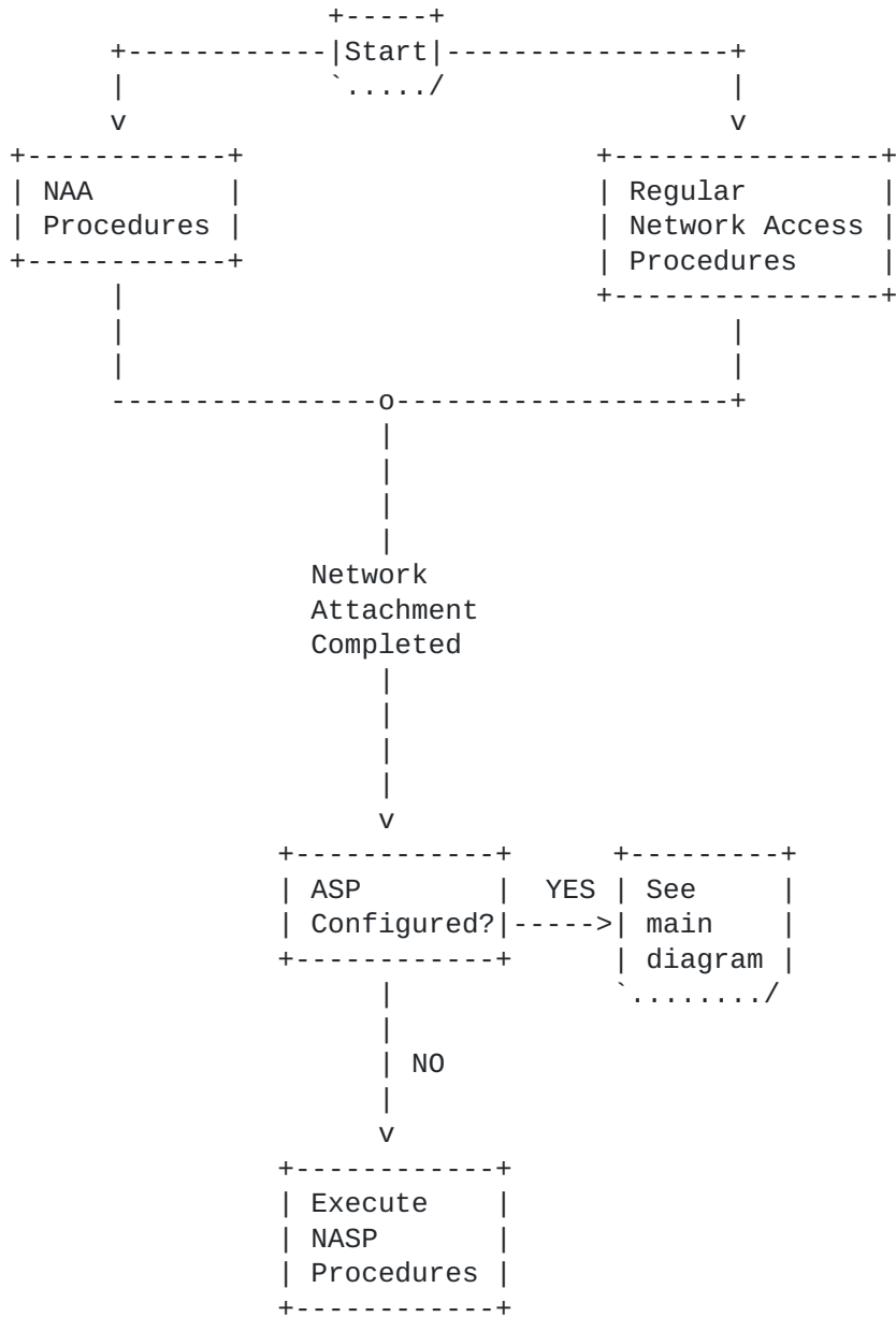
Figure 3: Flow Diagram: ZBP Scenario.
