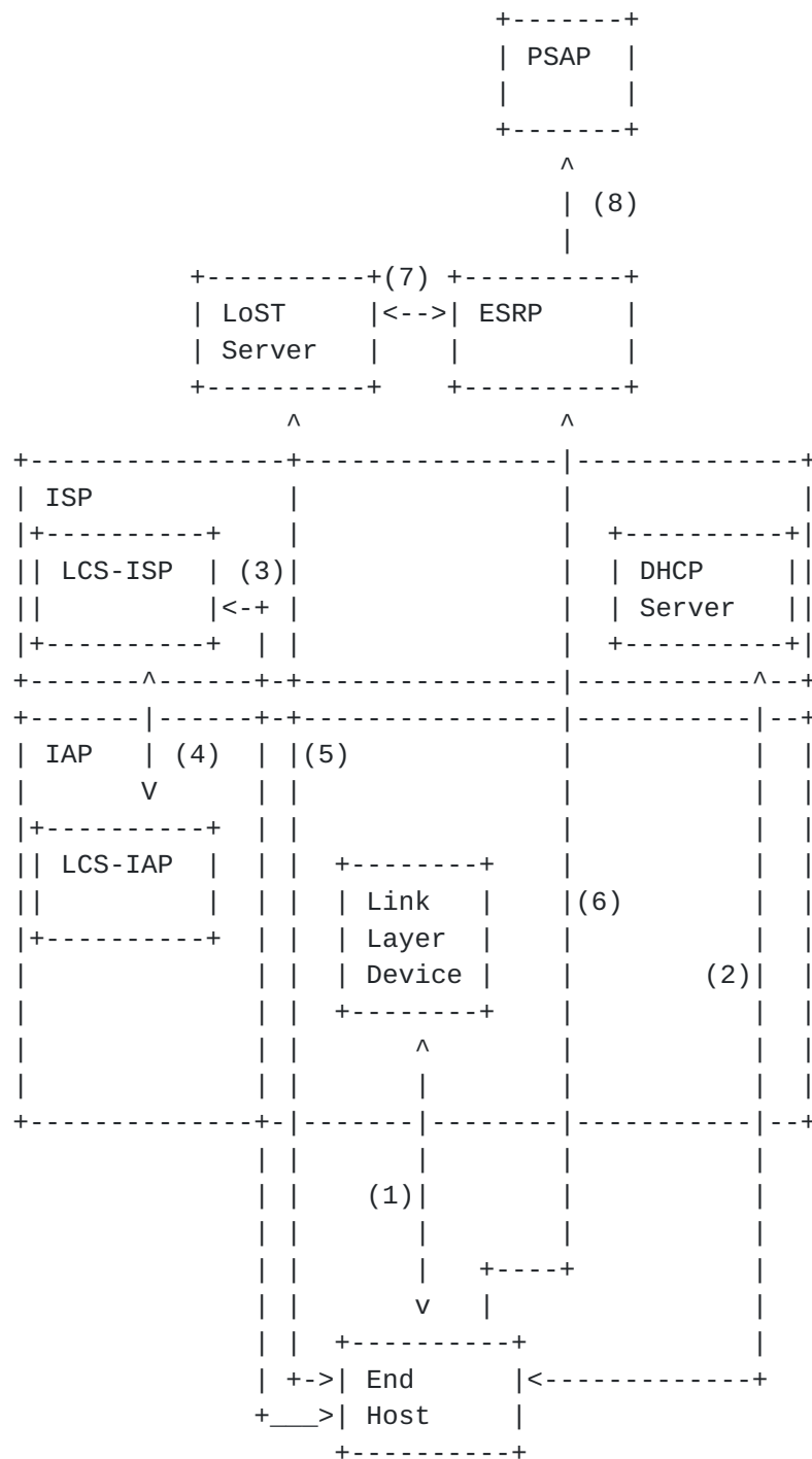
Figure 5: Architectural Overview
