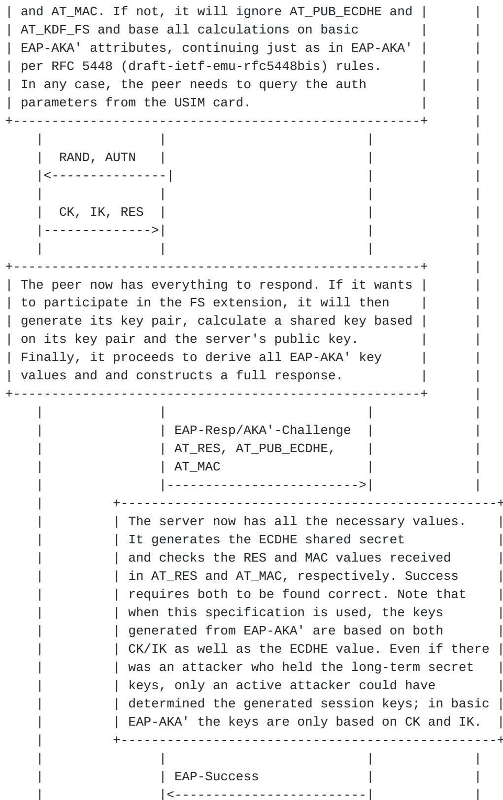
Figure 2: EAP-AKA' FS Authentication Process
