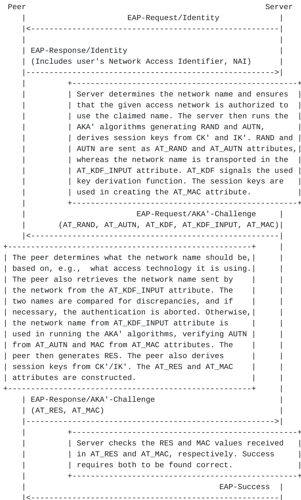
Figure 1: EAP-AKA' Authentication Process
