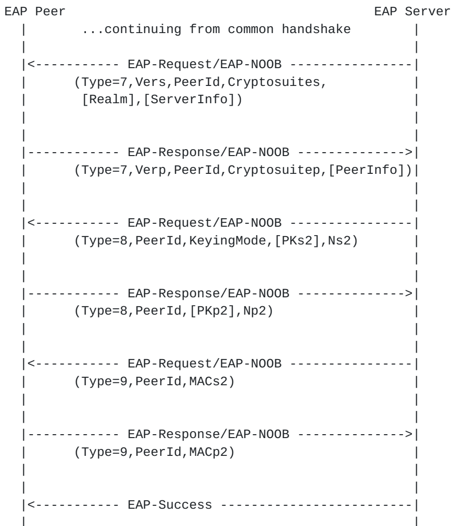
Figure 8: Reconnect Exchange
