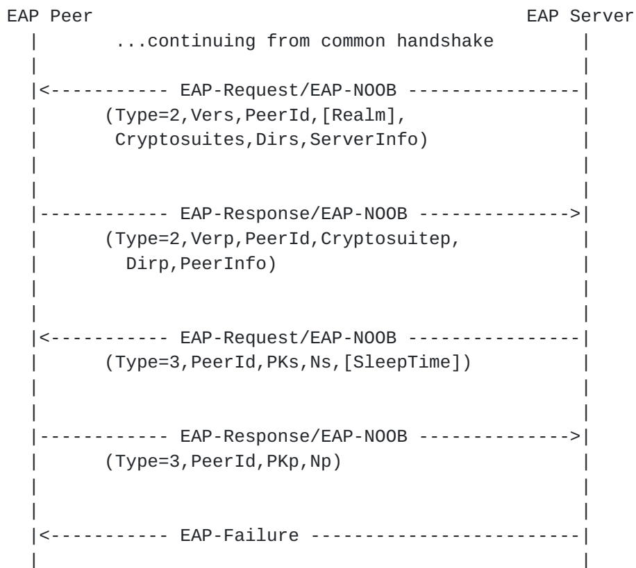
Figure 3: Initial Exchange
