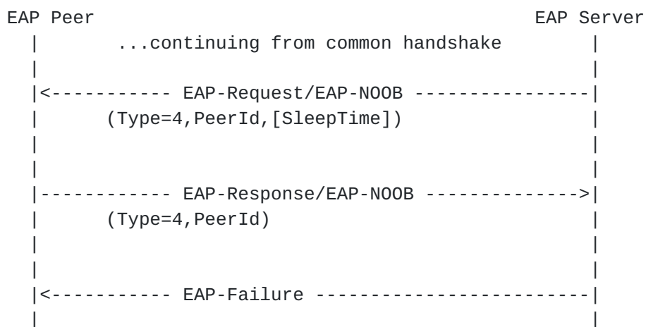
Figure 7: Waiting Exchange
