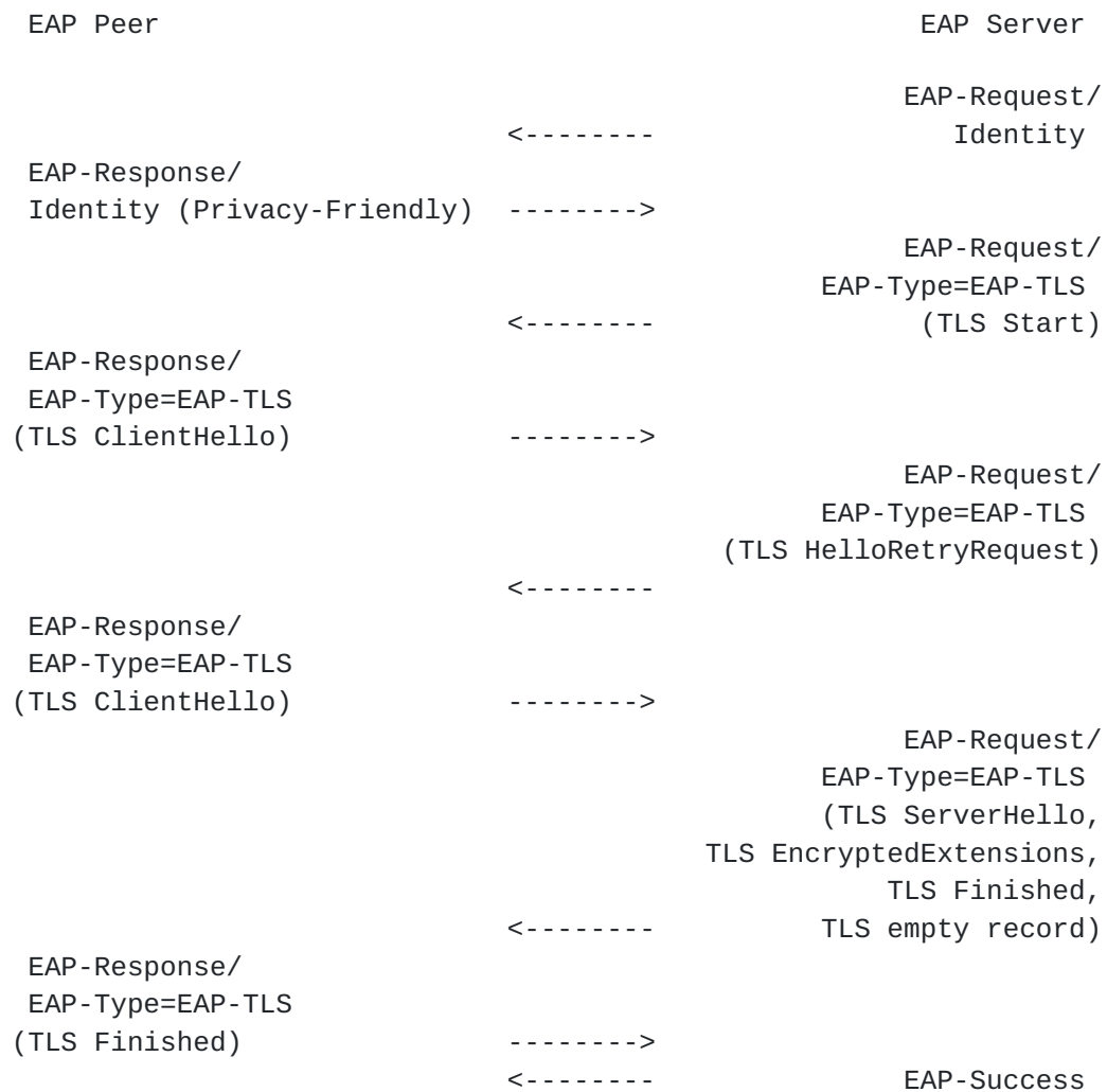
Figure 6: EAP-TLS with Hello Retry Request
