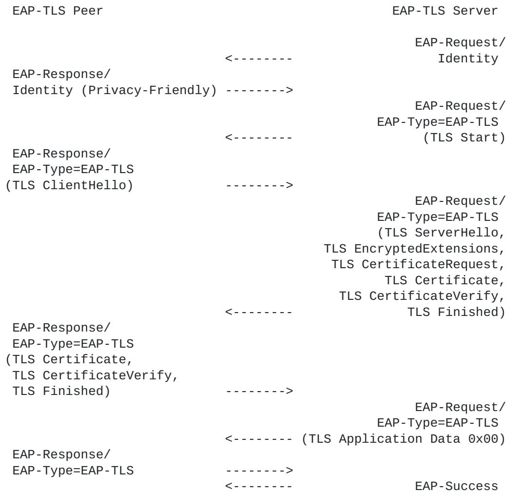
Figure 1: EAP-TLS mutual authentication
