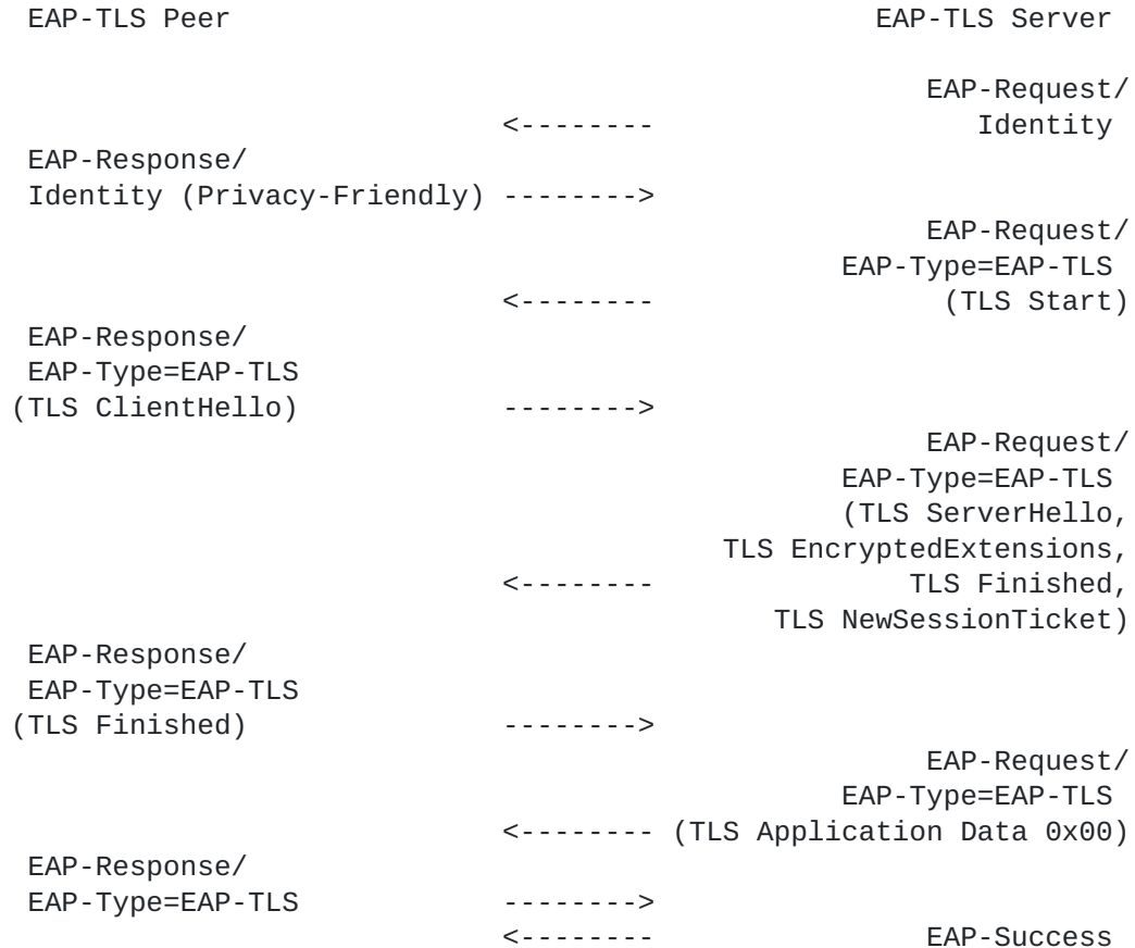
Figure 3: EAP-TLS resumption
