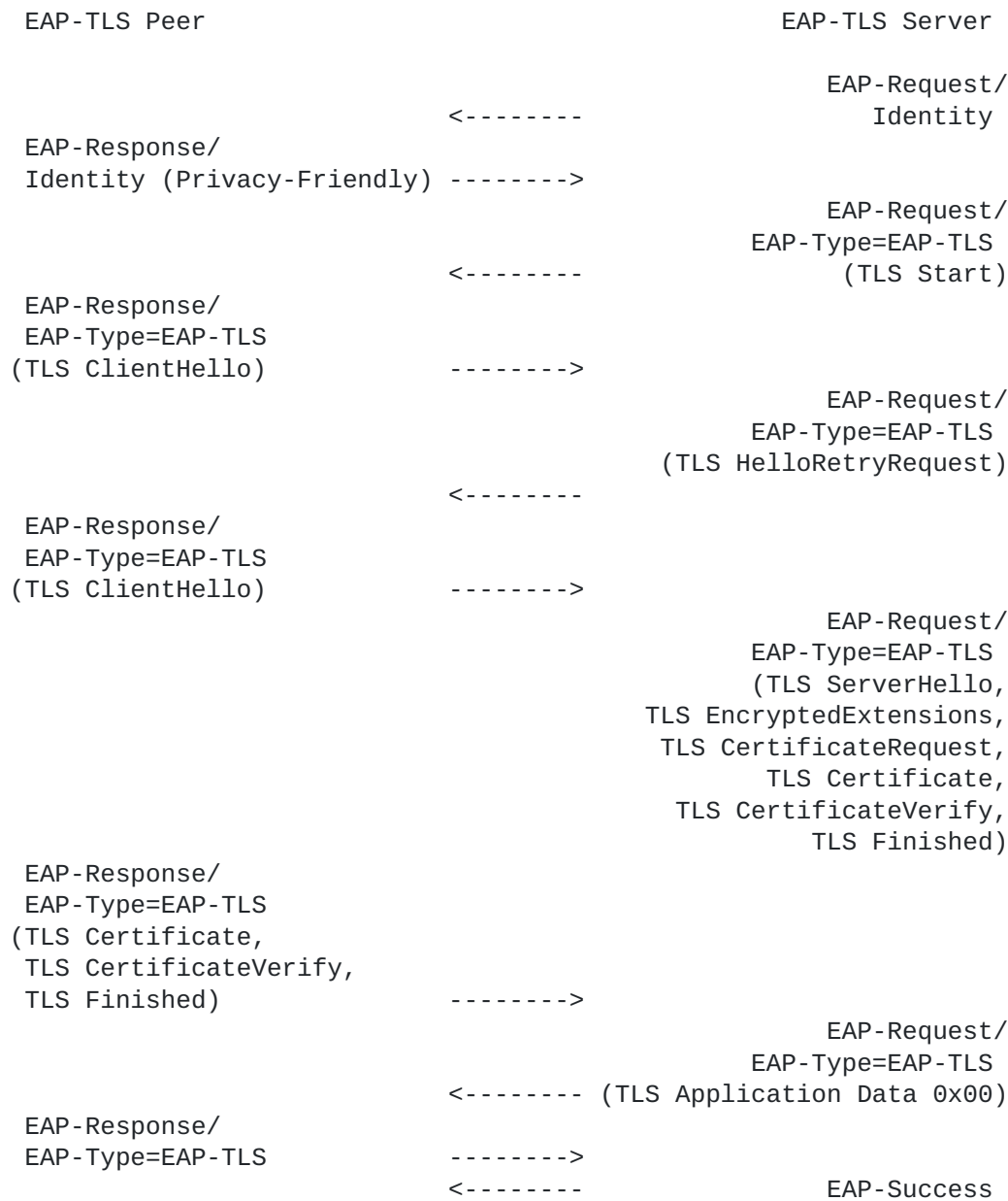
Figure 8: EAP-TLS with Hello Retry Request
