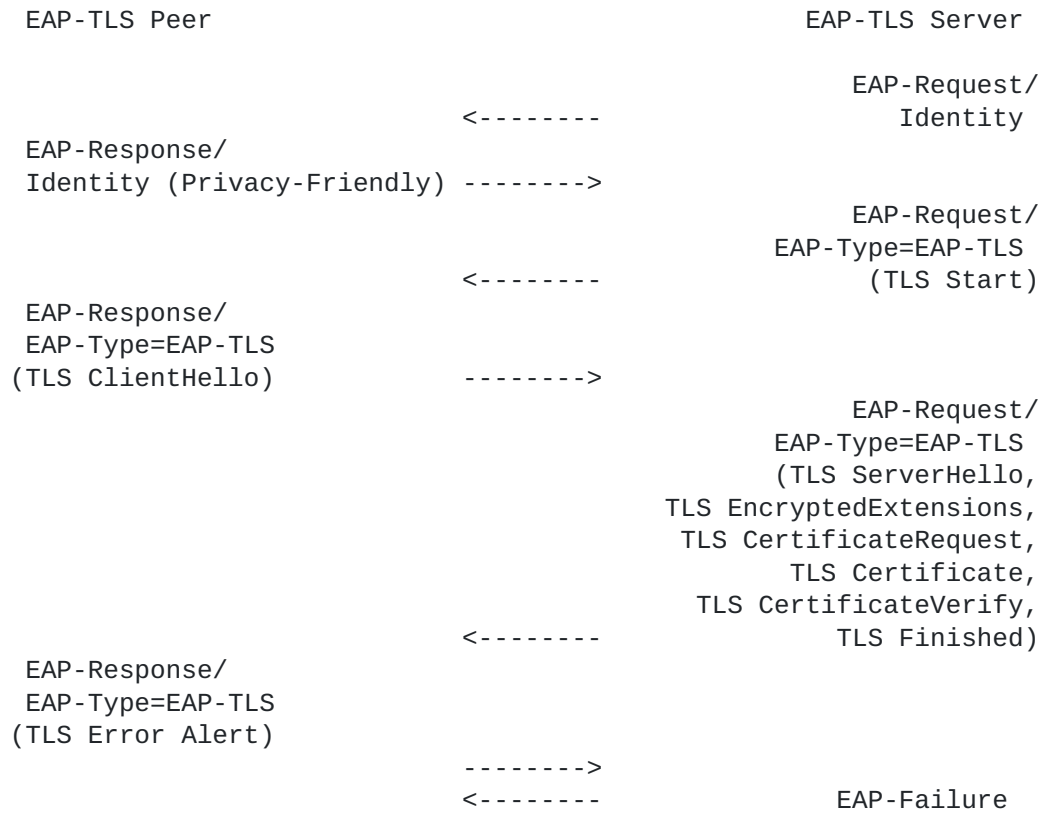
Figure 5: EAP-TLS unsuccessful EAP-TLS server authentication
