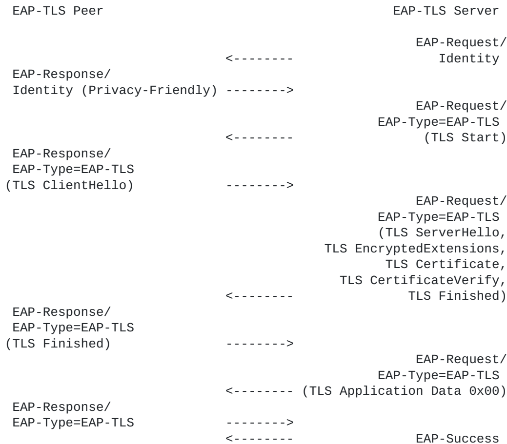
Figure 7: EAP-TLS without peer authentication
