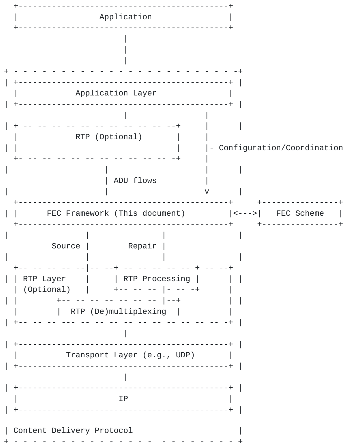
Figure 1: FEC Framework architecture
