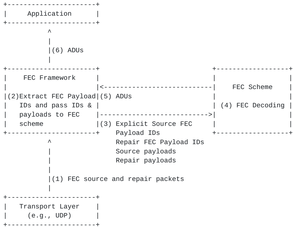
Figure 4: Receiver operation
