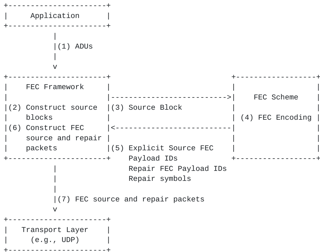
Figure 2: Sender operation
