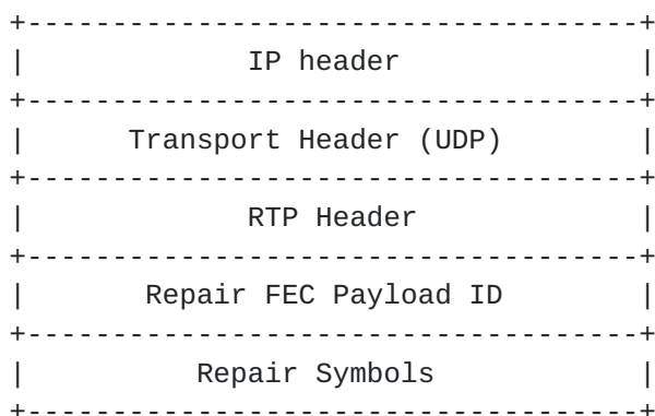
Figure 8: Packet format for repair packets
