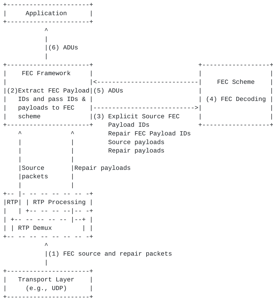
Figure 5: Receiver operation with RTP repair flows
