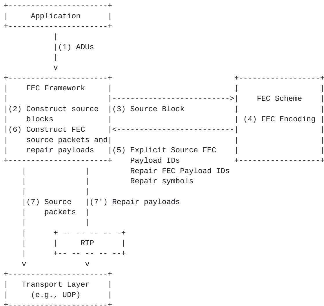
Figure 3: Sender operation with RTP repair flows
