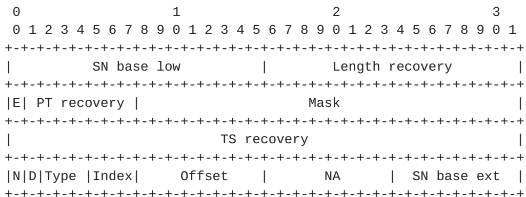
Figure 7: Format of the FEC header
