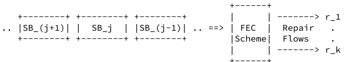
Figure 3: Repair flow generation by an FEC scheme
