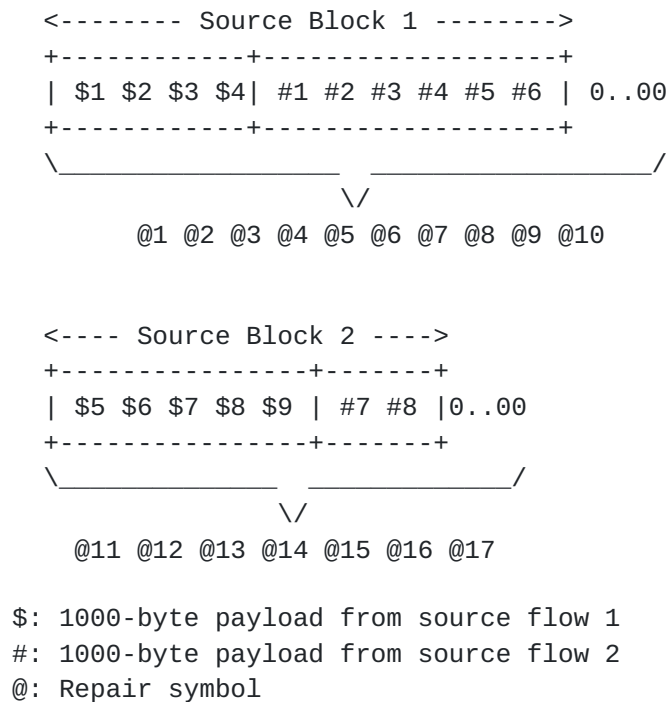
Figure 6: Source block with two source flows
