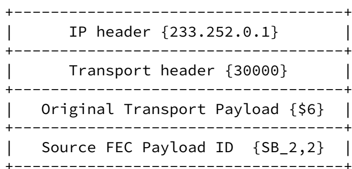
Figure 7: Example of a source packet for IPv4
