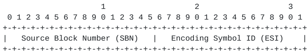
Figure 2: Source FEC Payload ID - Format A
