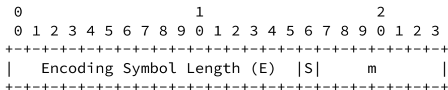
Figure 3: FSSI encoding format.
