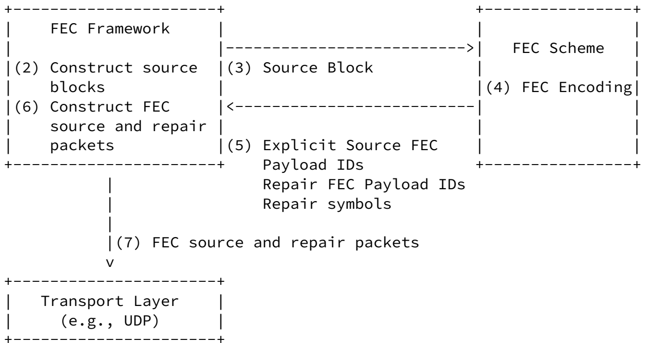
Figure 1: Terminology used in this document (sender).
