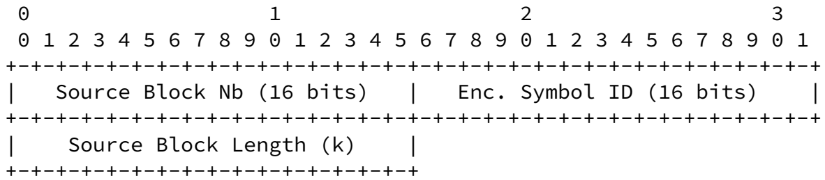
Figure 6: Source FEC Payload ID encoding format for m = 16.
