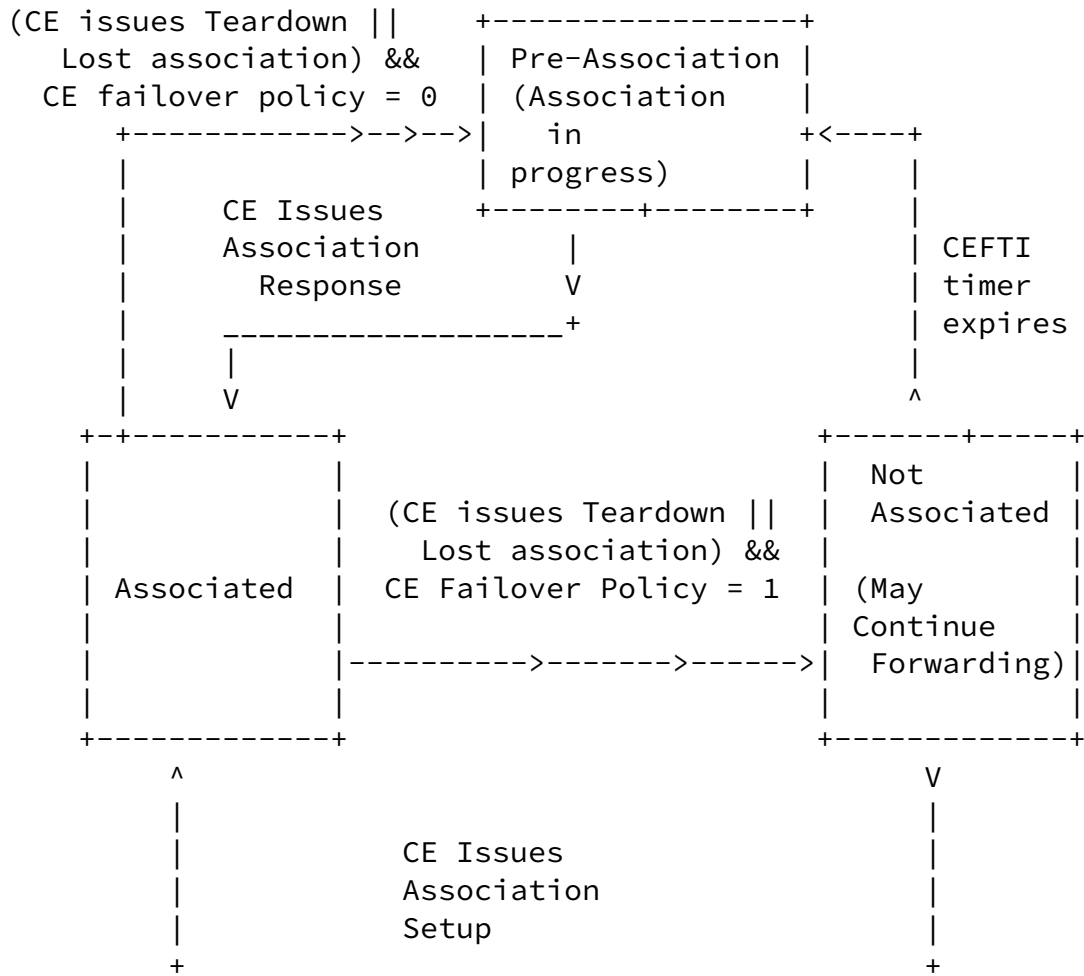
Figure 3: FE State Machine considering HA
