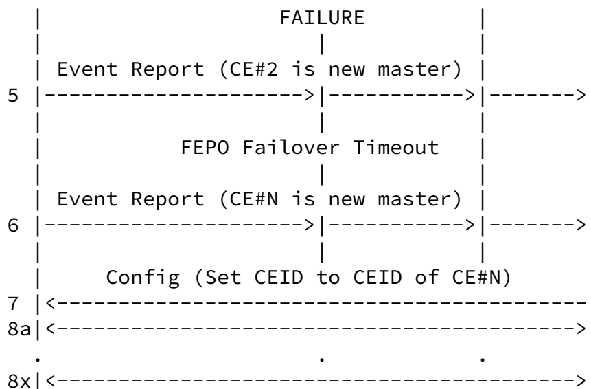
Figure 5: CE Failover for Hot Standby
