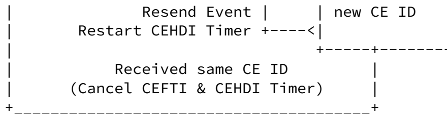
Figure 4: FE State Machine considering HA
