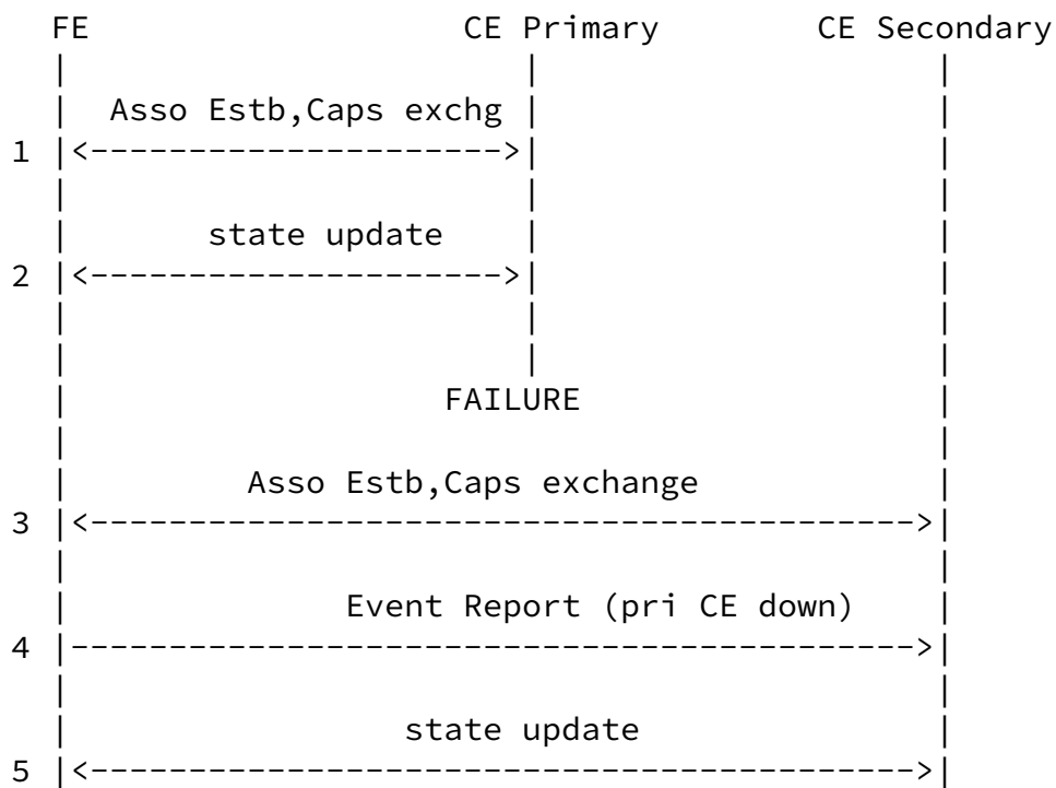
Figure 2: CE Failover for Cold Standby
