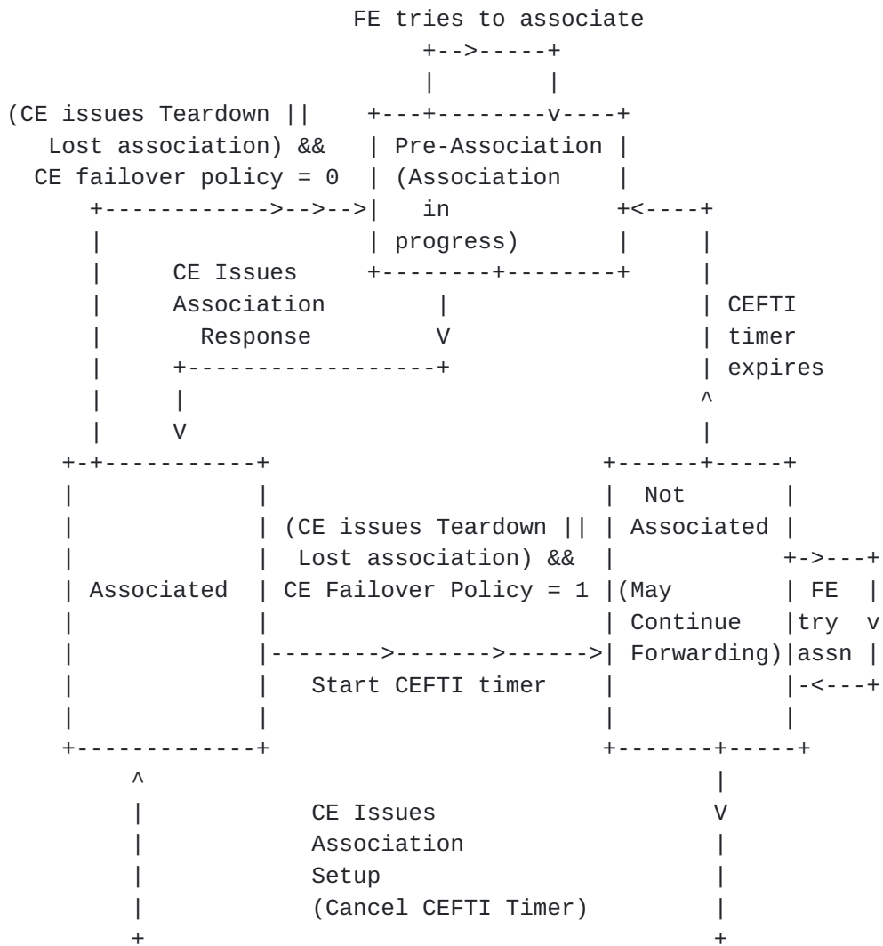
Figure 3: FE State Machine considering HA
