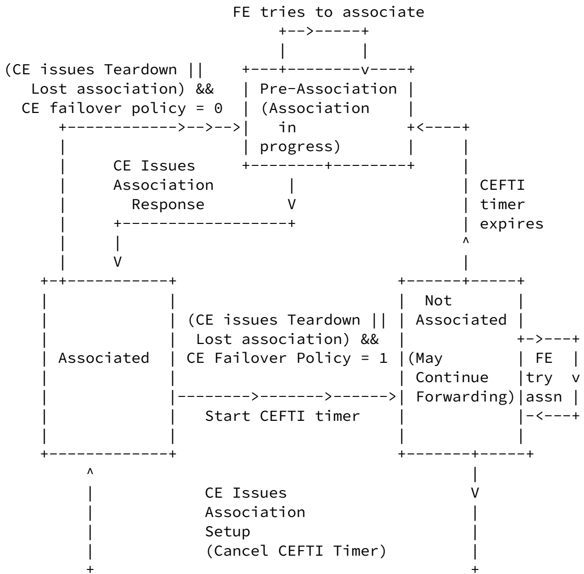
Figure 3: FE State Machine considering HA
