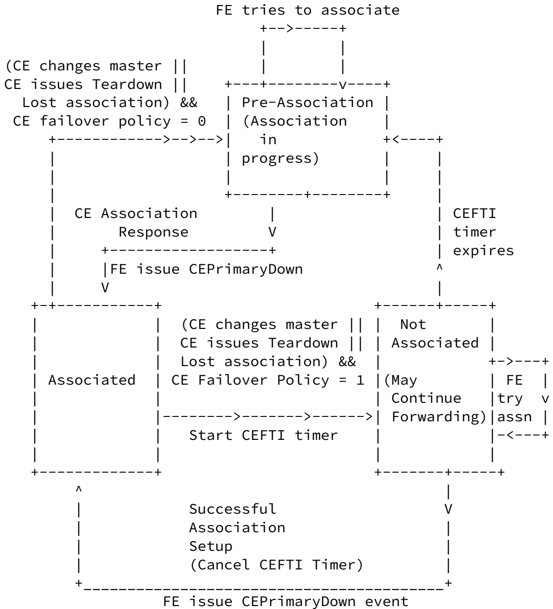
Figure 3: FE State Machine considering HA
