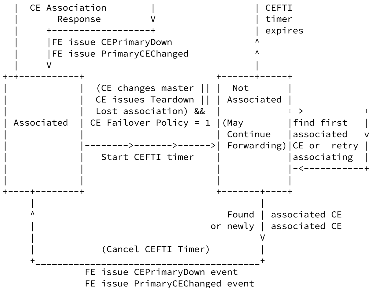
Figure 4: FE State Machine considering HA
