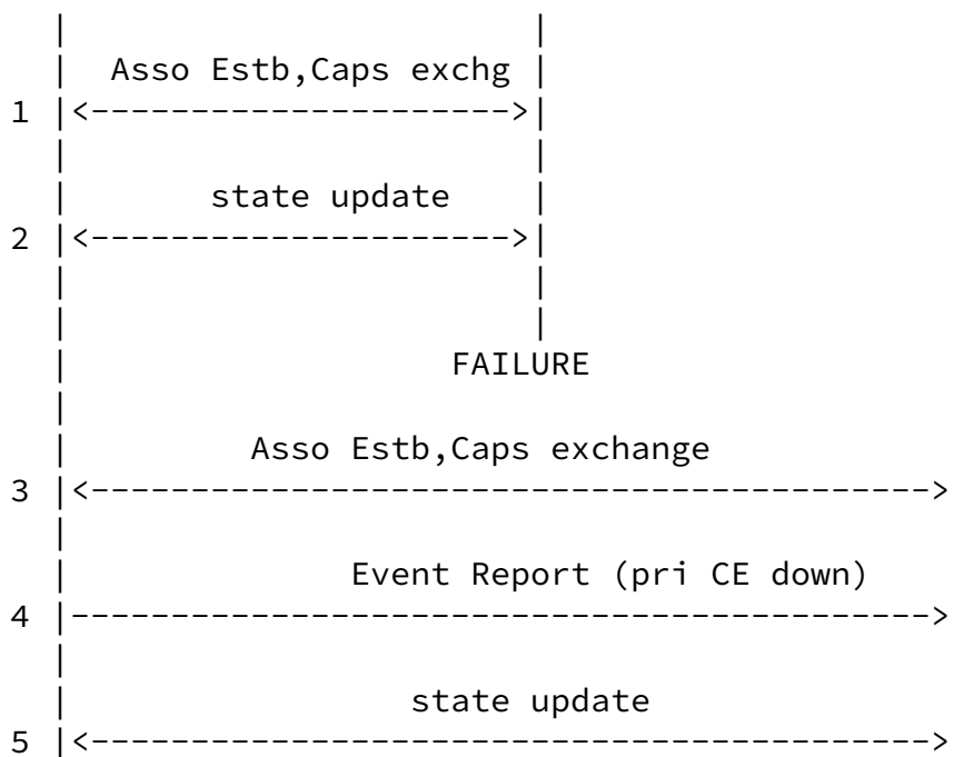
Figure 2: CE Failover for Cold Standby
