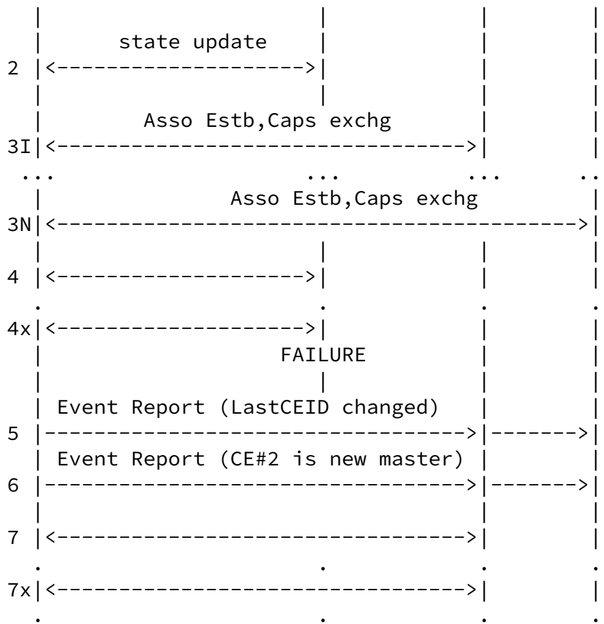
Figure 5: CE Failover for Hot Standby
