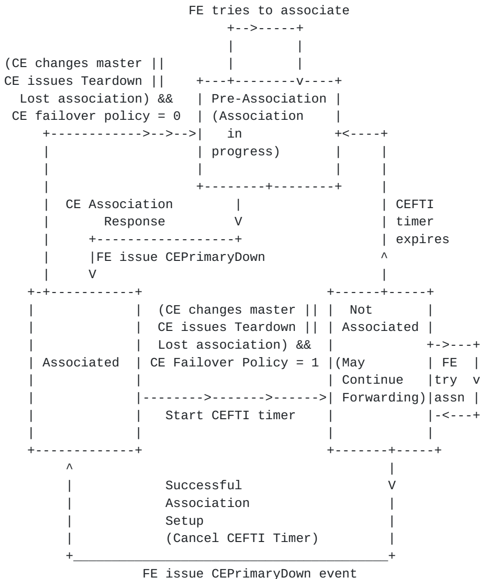
Figure 3: FE State Machine considering HA
