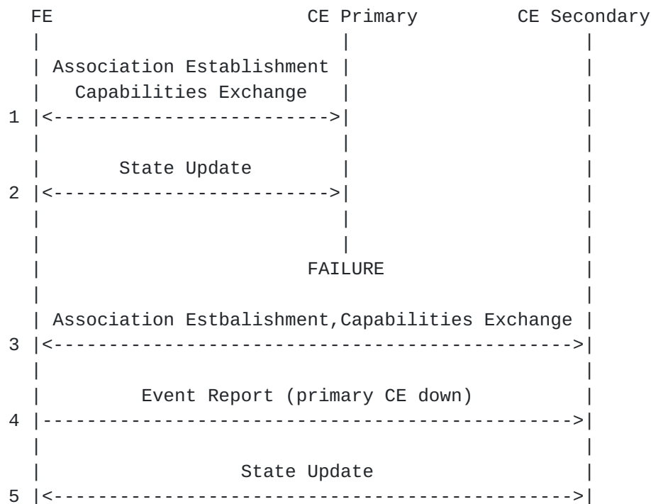
Figure 2: CE Failover for Cold Standby
