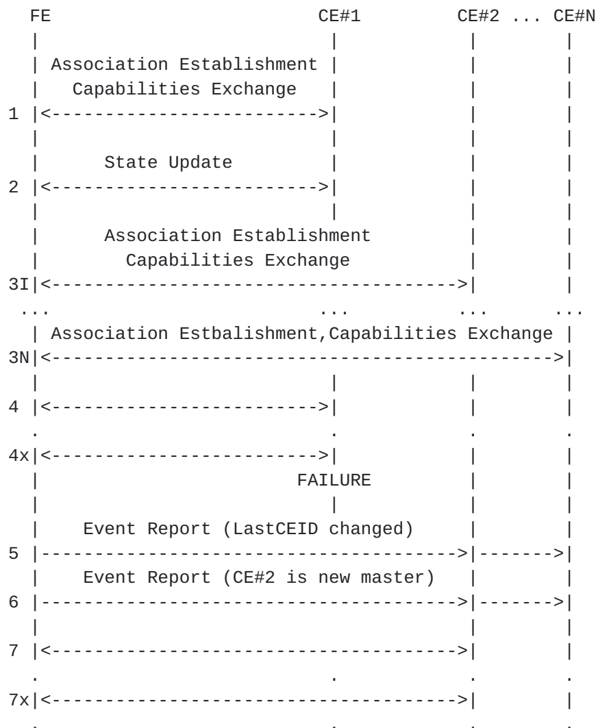
Figure 5: CE Failover for Hot Standby
