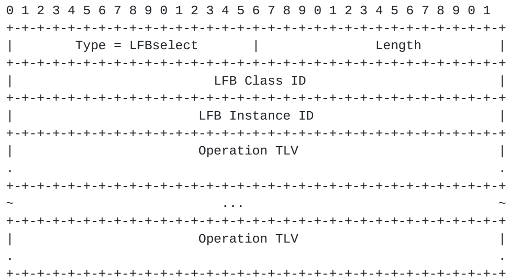
Figure 13: PL PDU layout
