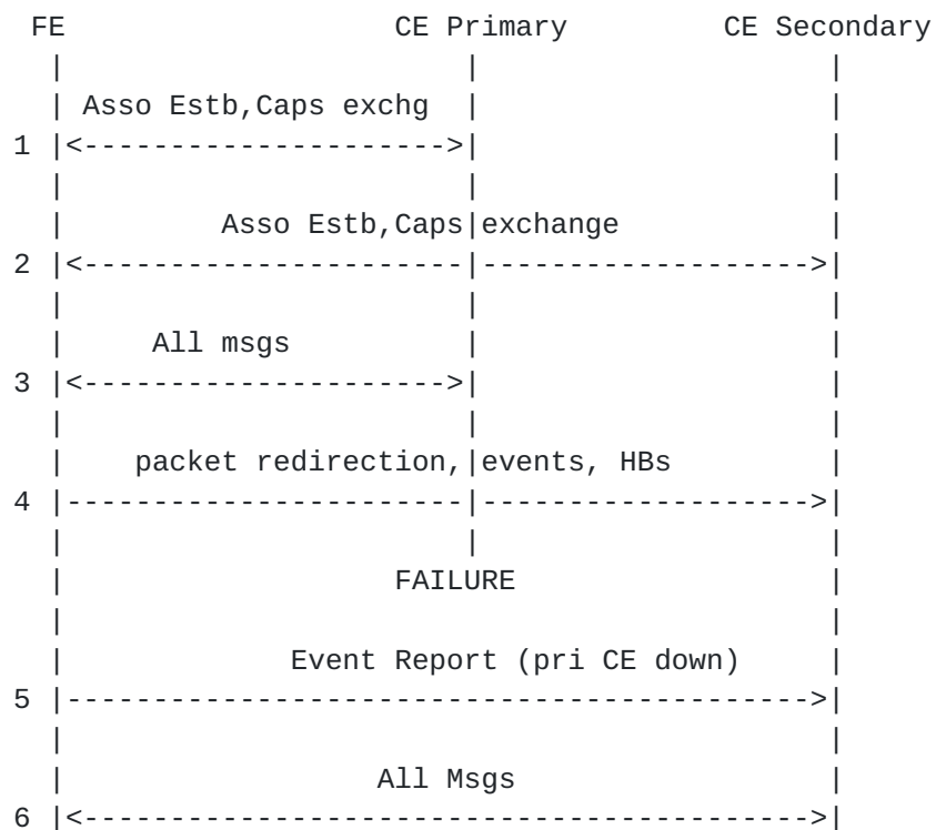
Figure 34: CE Failover for Report All mode
