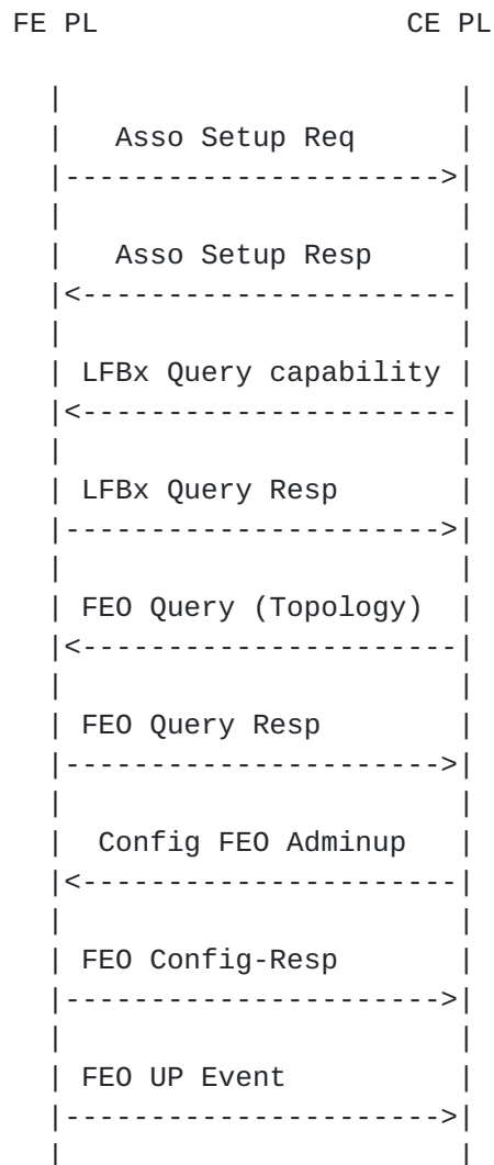
Figure 32: Message exchange between CE and FE to establish an NE association
