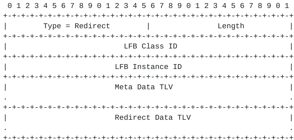
Figure 28: Redirect_Data TLV
