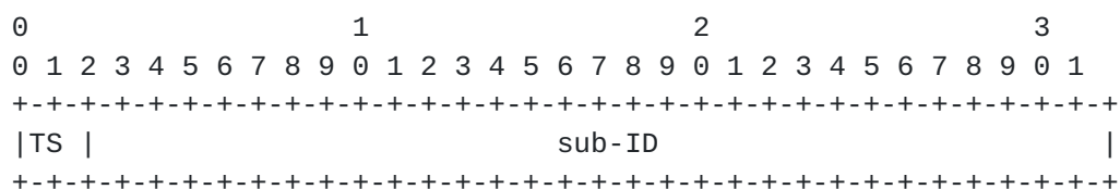
Figure 8: ForCES ID Format
