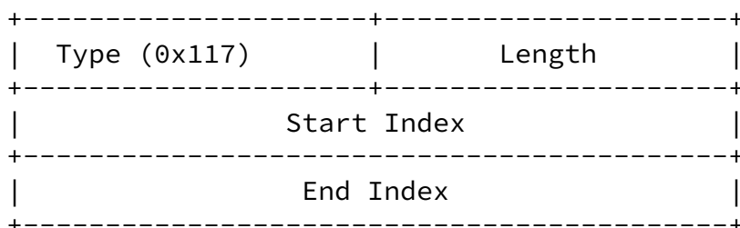
Figure 1: ForCES table range request Layout
