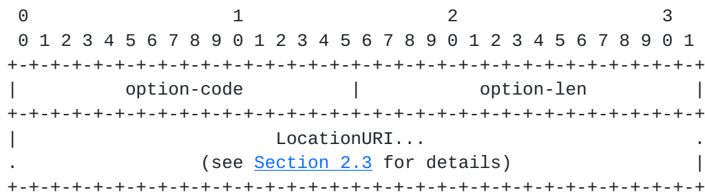
Figure 2. IPv6 fields of this LocationURI Option
