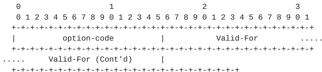
Figure 2. IPv6 fields of this Valid-For Option
