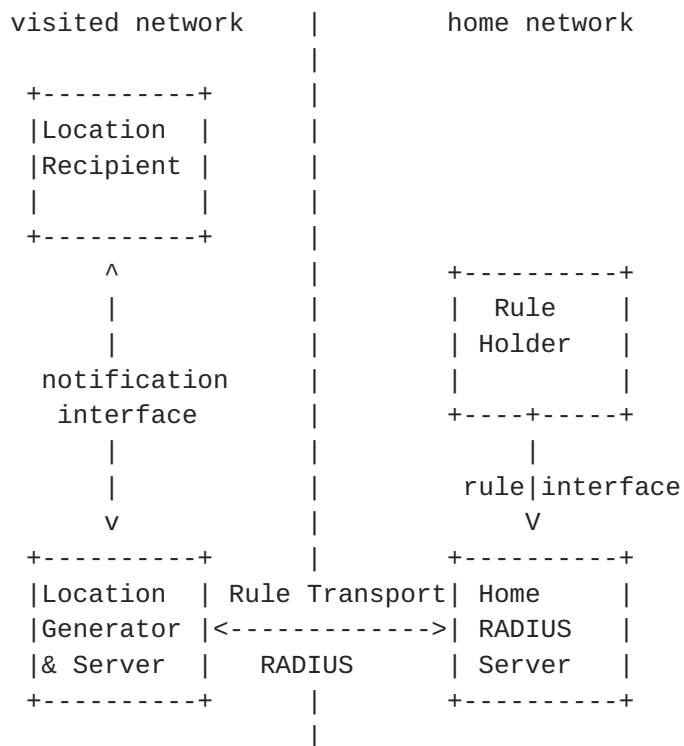
Figure 19: Location Server at the Visited Network
