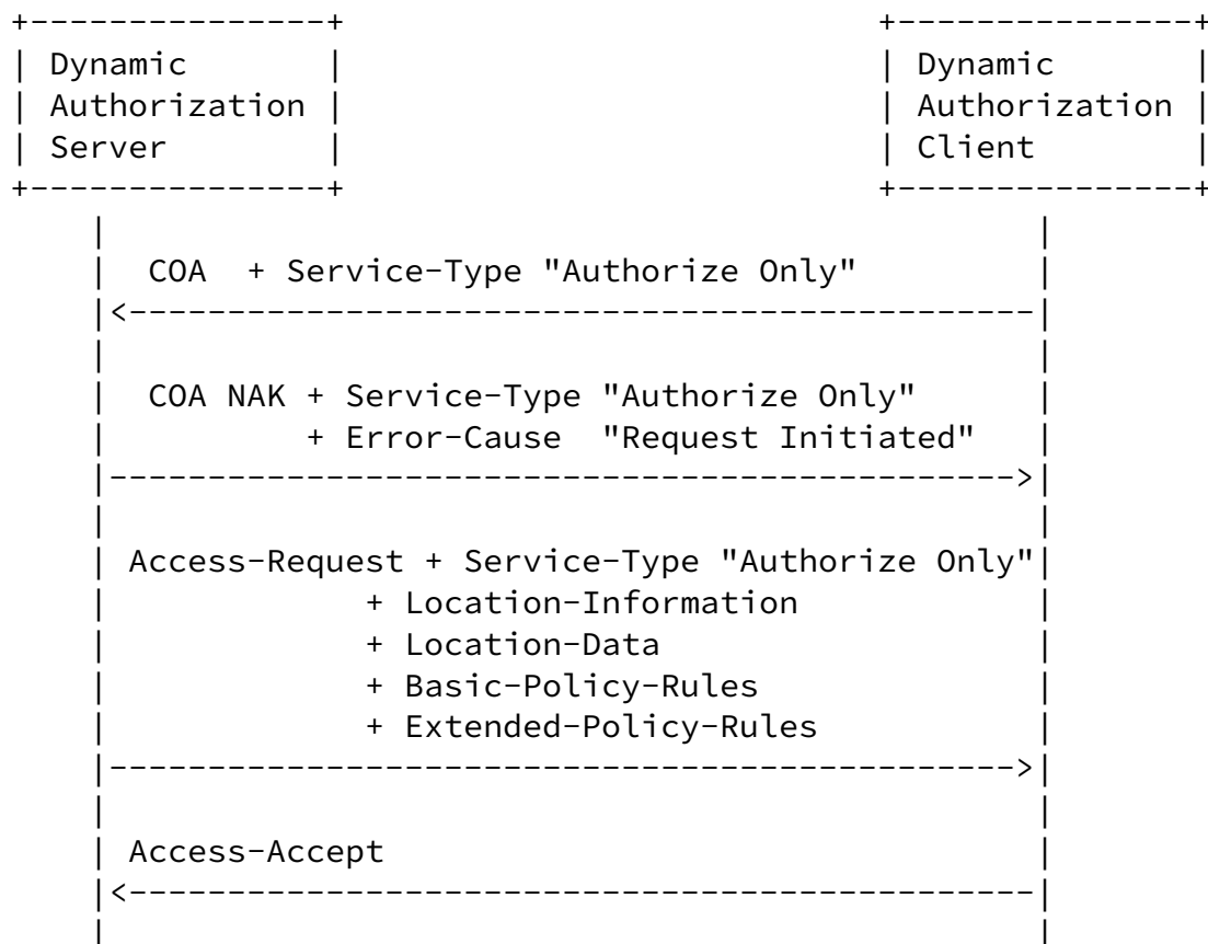
Figure 3: Location Delivery based on Mid-Session Request
