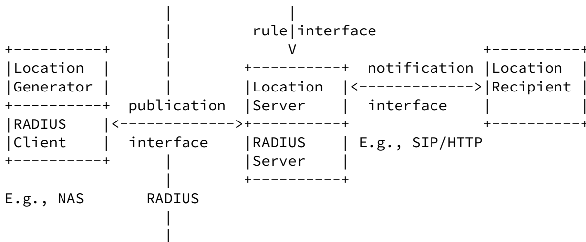
Figure 18: Location Server at the Home Network
