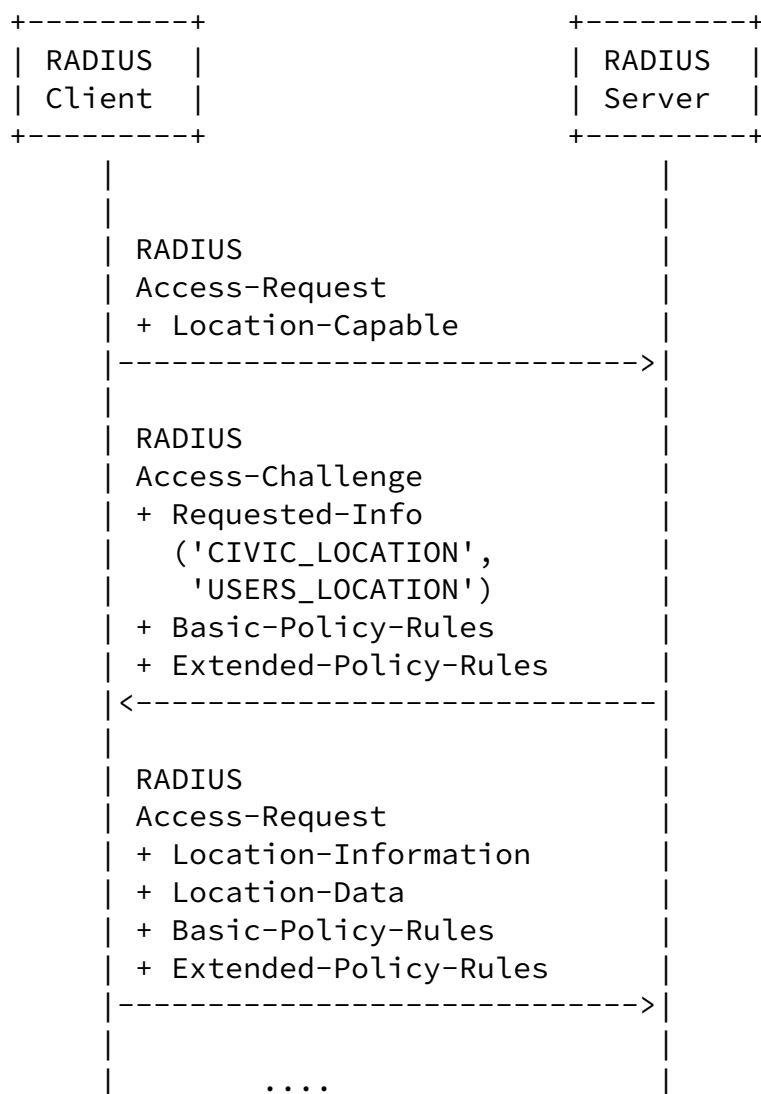
Figure 11: RADIUS server requesting location information
