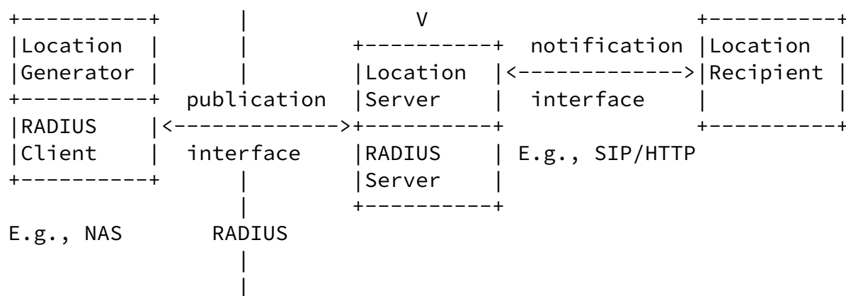
Figure 19: Location Server at the Home Network
