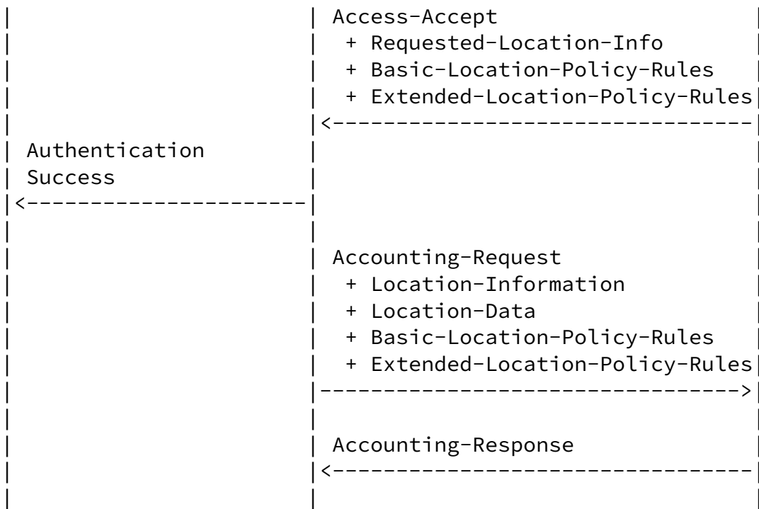
Figure 5: Location Delivery in Accounting Messages
