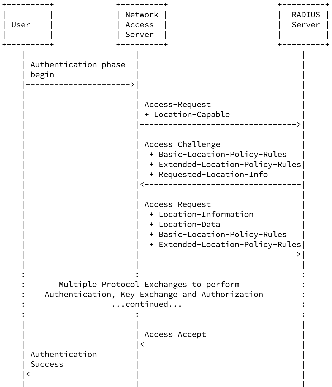
Figure 2: Location Delivery based on Initial Request
