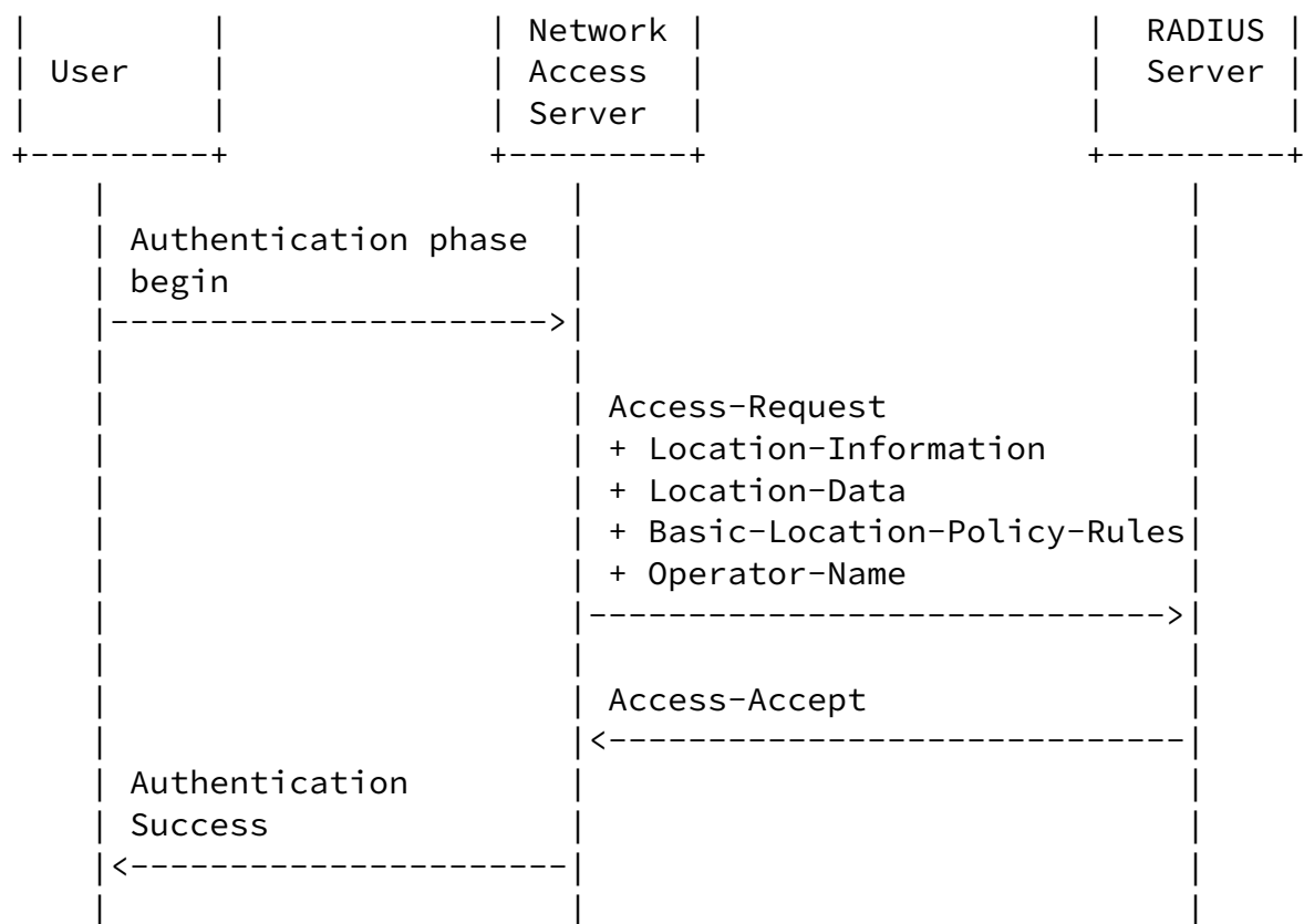
Figure 1: Location Delivery based on out-of-band Agreements
