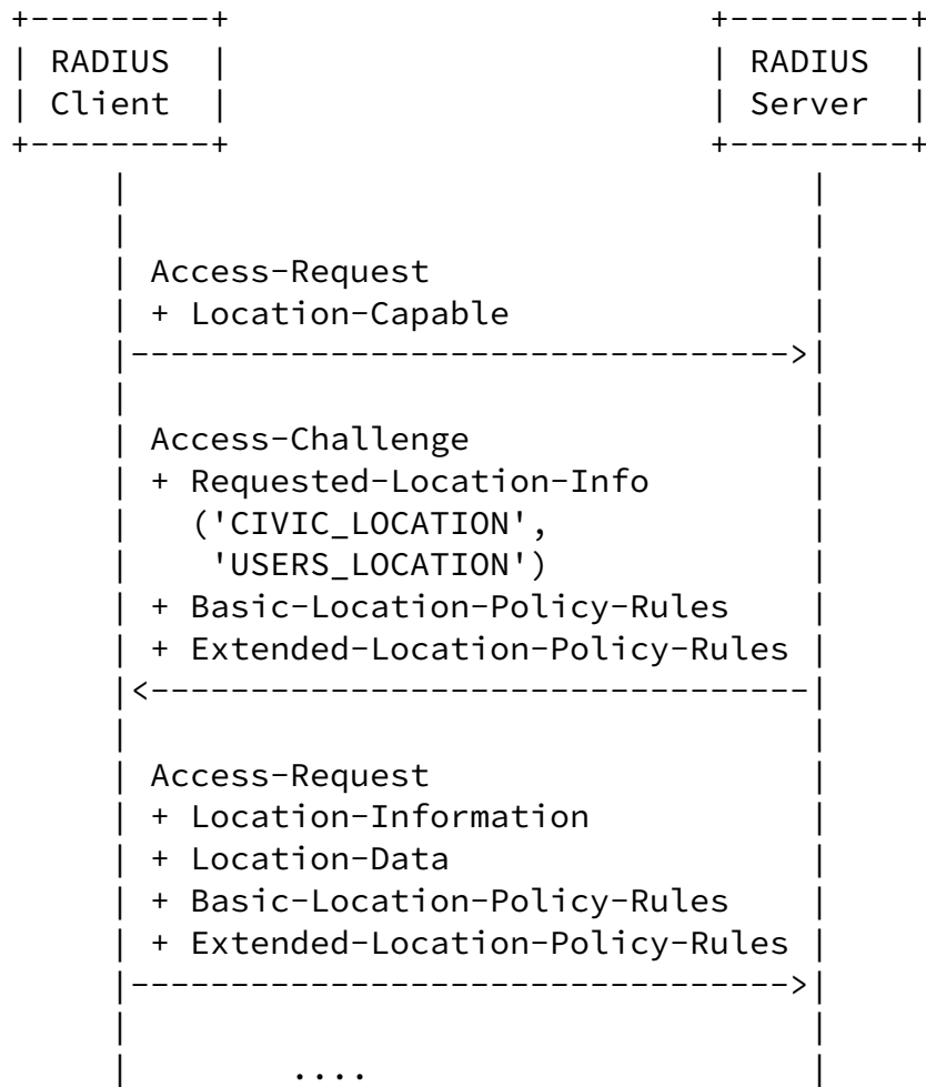
Figure 6: RADIUS server requesting location information
