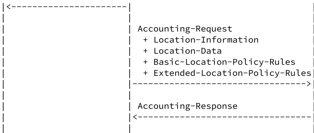
Figure 5: Location Delivery in Accounting Messages
