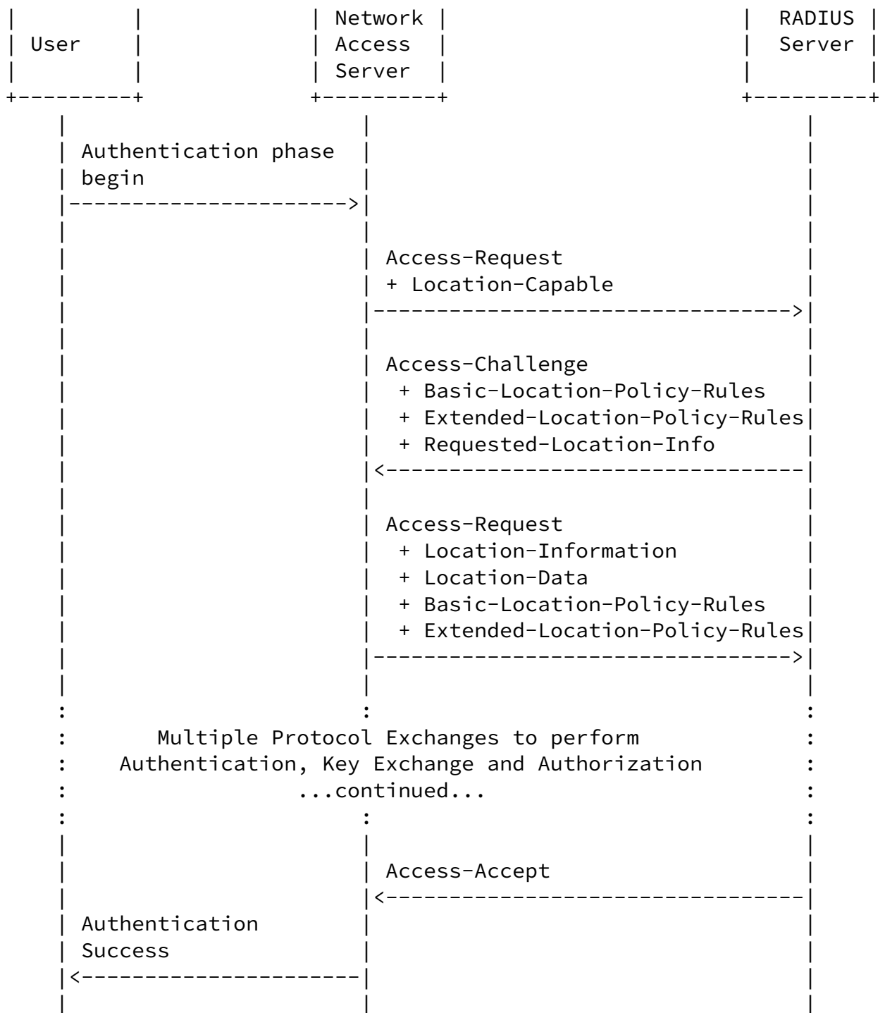
Figure 2: Location Delivery based on Initial Request
