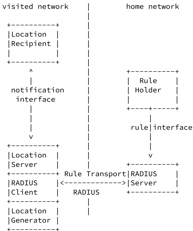
Figure 9: Location Server at the Visited Network
