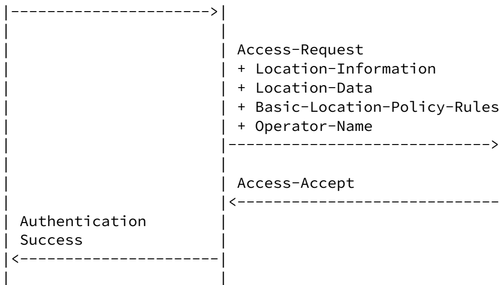
Figure 1: Location Delivery based on out-of-band Agreements
