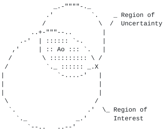
Figure 7: Area of Overlap Between Two Circular Regions
