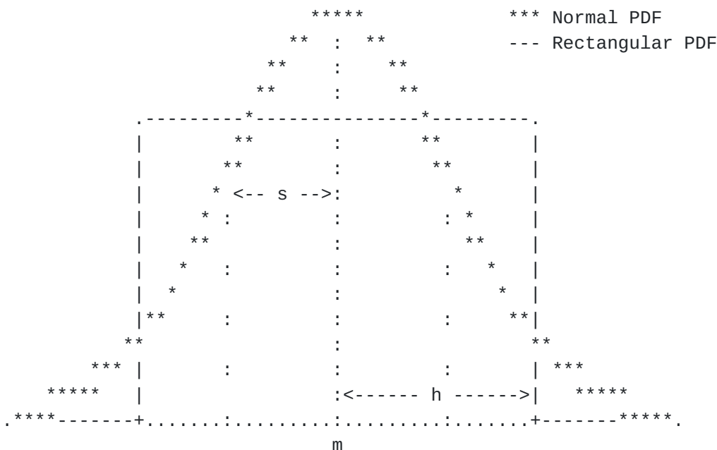
Figure 1: Normal and Rectangular Probability Density Functions
