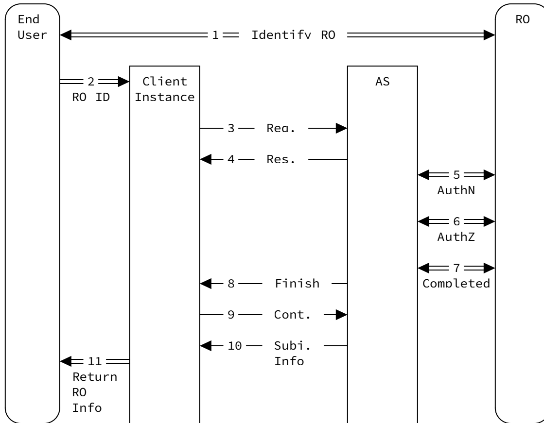
Figure 10: Figure 10: Diagram of cross-user authorization, where the end user and RO are different
