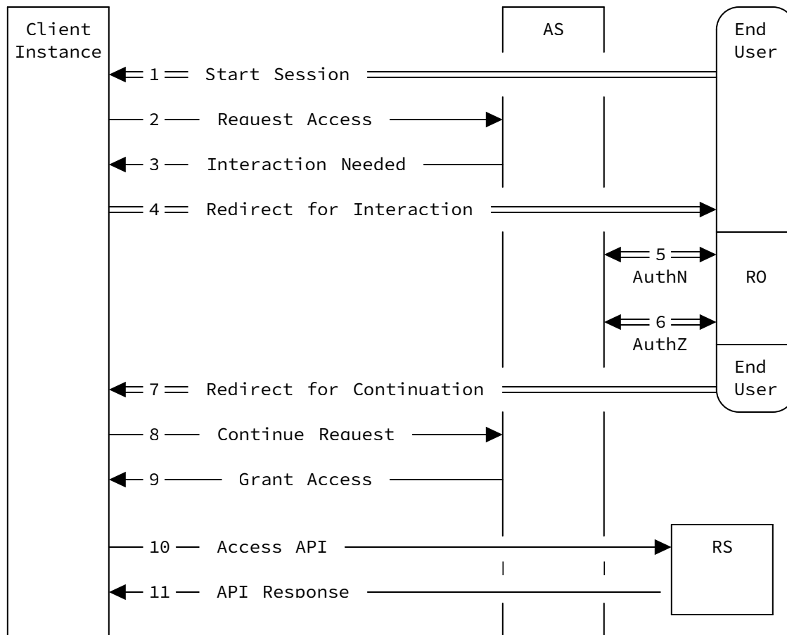
Figure 4: Figure 4: Diagram of a redirect-based interaction
