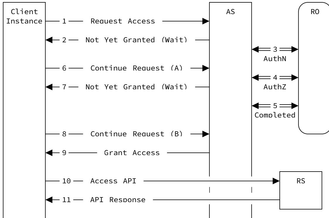
Figure 6: Figure 6: Diagram of an asynchronous authorization process, with no end user interaction
