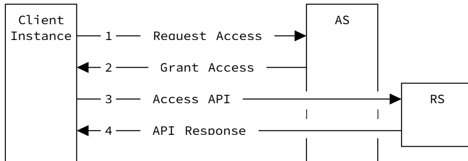
Figure 7: Figure 7: Diagram of a software-only authorization, with no end user or explicit resource owner
