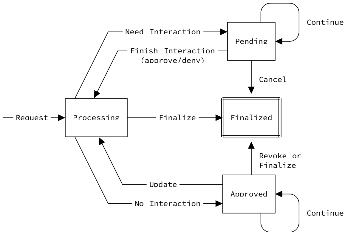
Figure 2: Figure 2: State diagram of a grant request throughout GNAP
