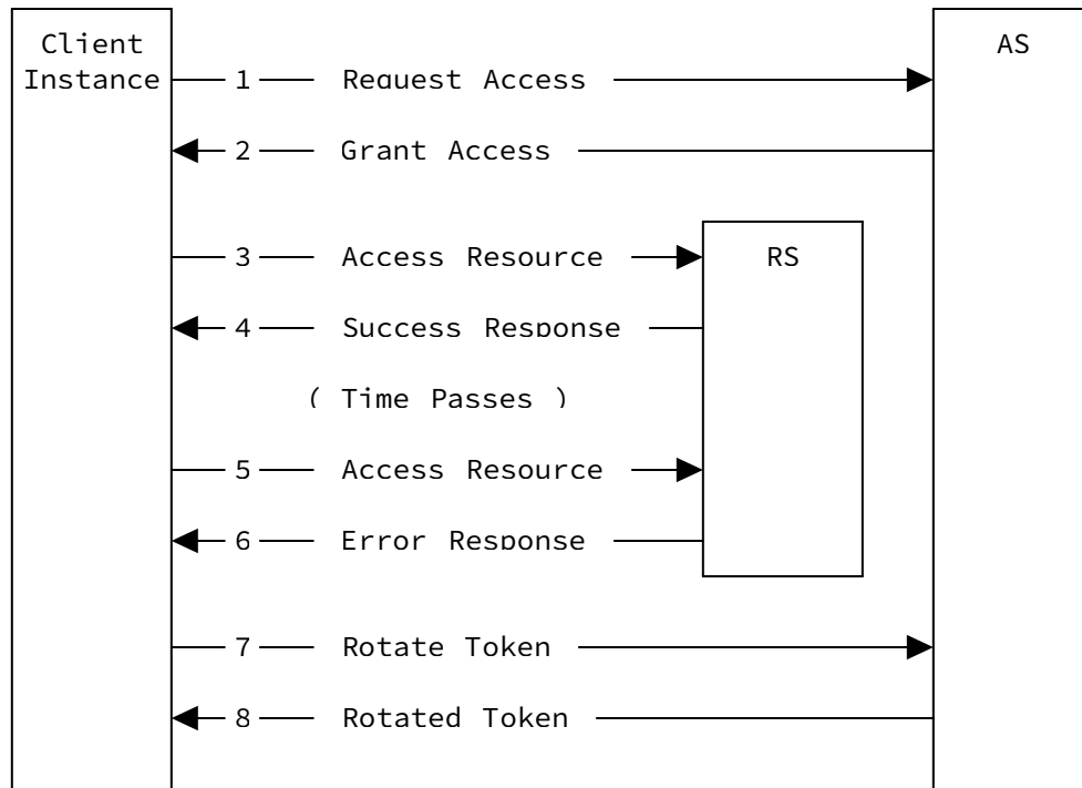
Figure 8: Figure 8: Diagram of the process of refreshing an access token
