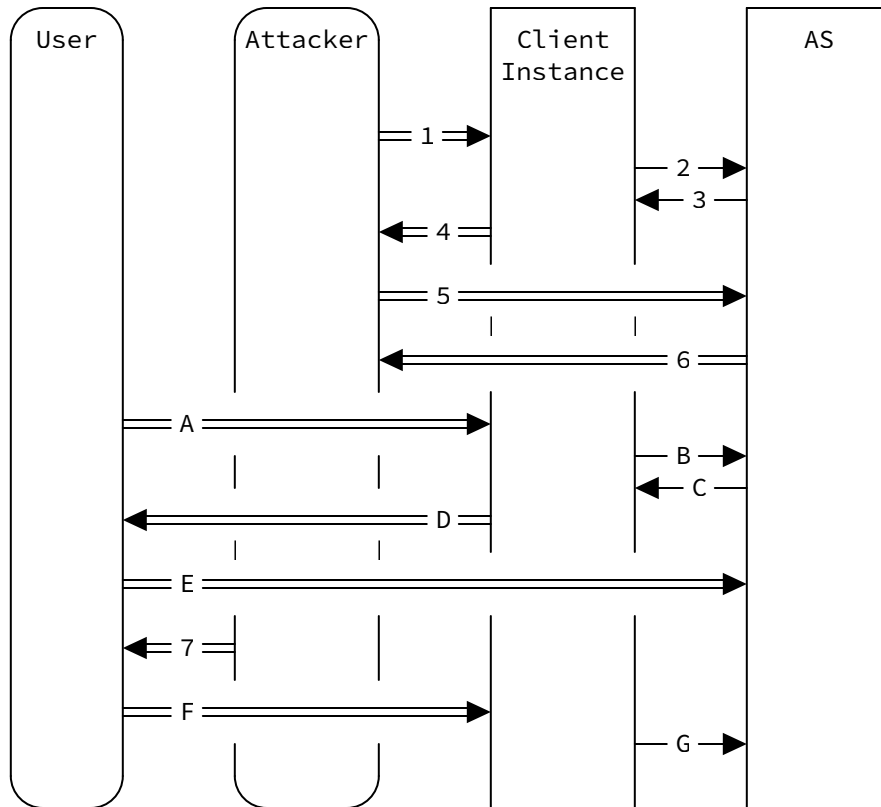
Figure 11: Figure 11: Interaction hash attack
