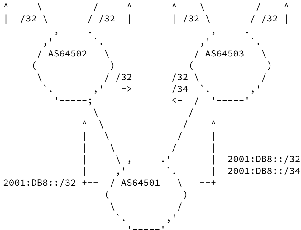
Figure 3: Remote triggered filtering
