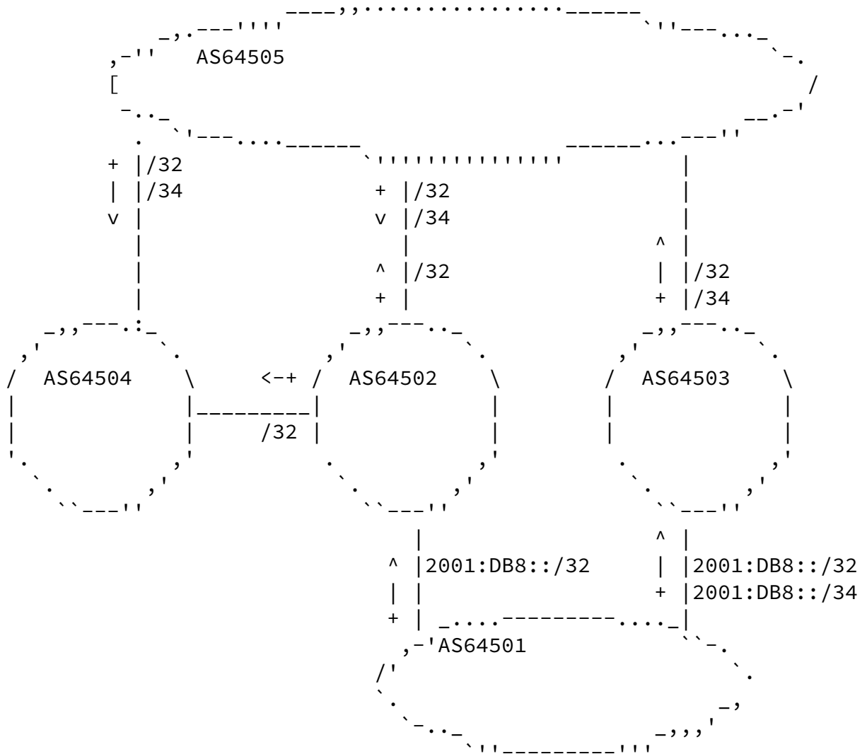
Figure 5: Traffic Engineering of unexpected traffic flows - Base example
