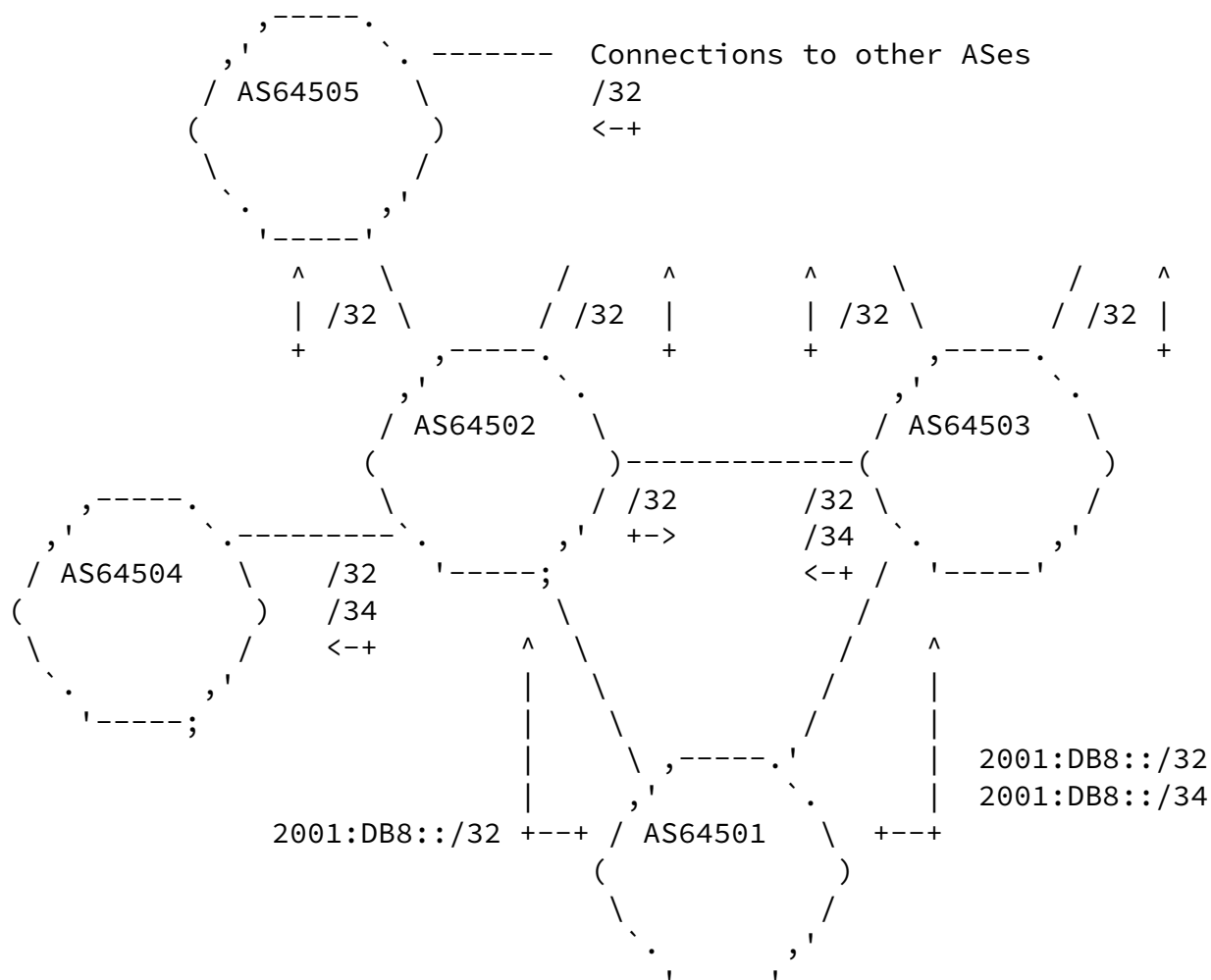
Figure 4: Unexpected traffic flows due to remote triggered filtering
