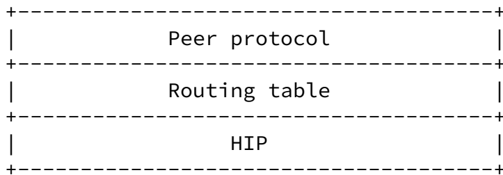
Figure 5: Routing tables
