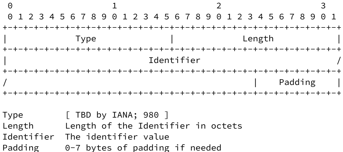
Figure 8: Format of the OVERLAY_ID Parameter
