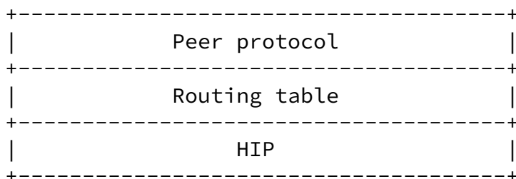
Figure 6: Routing Tables
