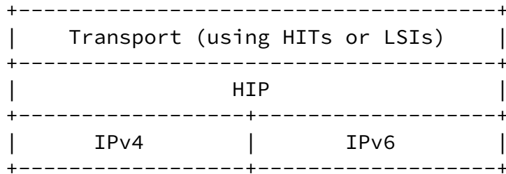
Figure 4: HIP as a Thin Waist
