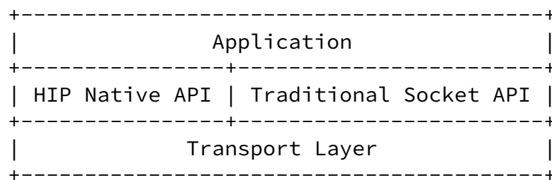
Figure 1: HIP API
