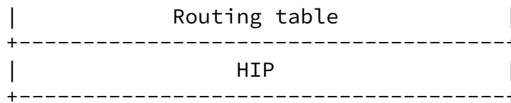
Figure 6: Routing Tables
