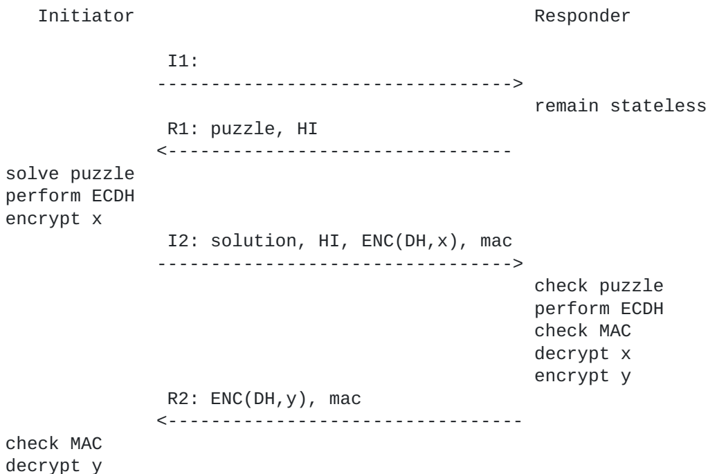
Figure 1: High-level overview of the HIP Diet EXchange
