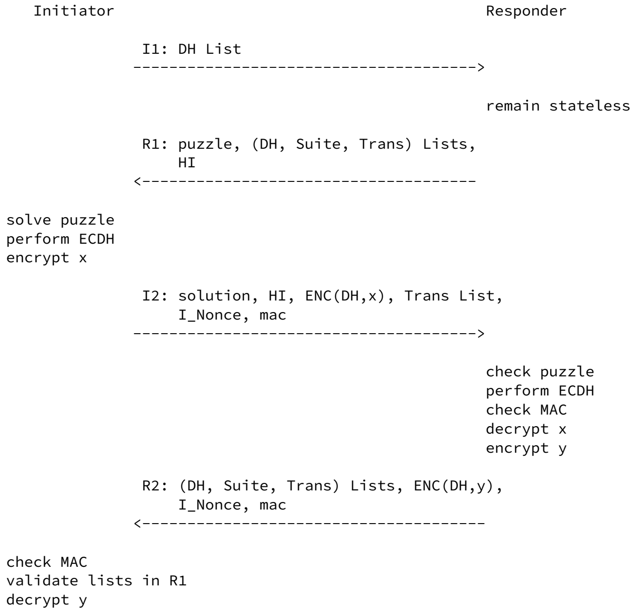
Figure 1: High-level overview of the HIP Diet EXchange
