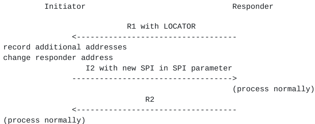
Figure 10: LOCATOR inclusion in R1
