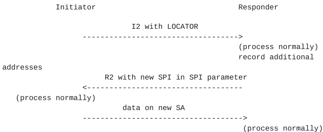
Figure 11: LOCATOR inclusion in I2
