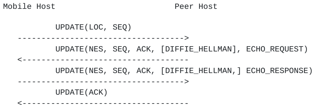
Figure 6: Readdress with peer-initiated rekey
