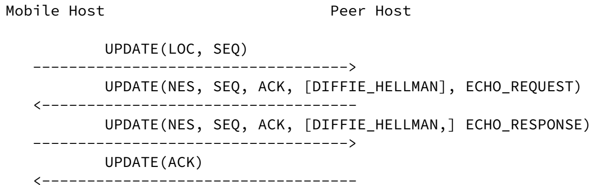
Figure 6: Readdress with peer-initiated rekey
