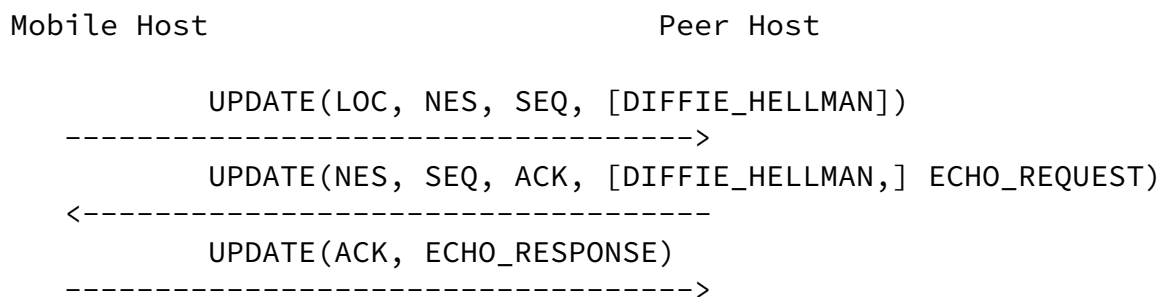
Figure 5: Readdress with mobile-initiated rekey
