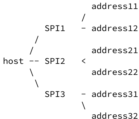
Figure 3: Relation between hosts, SPIs, and addresses (general case)
