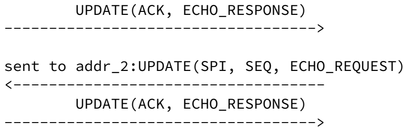
Figure 8: LOCATOR with multiple addresses
