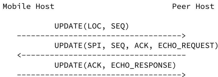
Figure 4: Readdress without rekeying, but with address check
