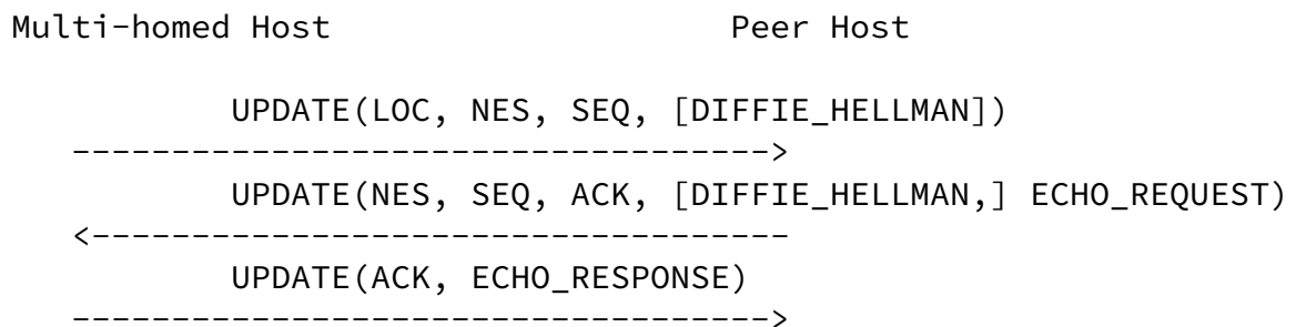
Figure 7: Basic multihoming scenario
