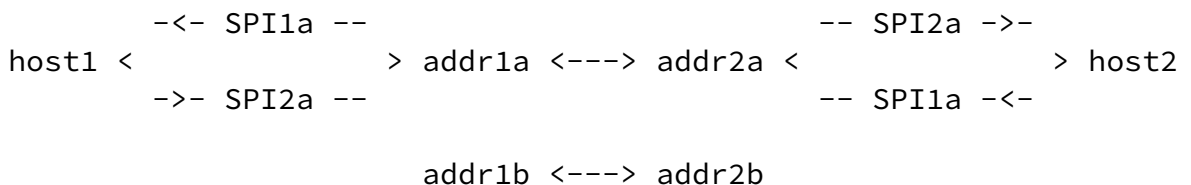
Figure 9: Dual multihoming case in which each host uses LOCATOR to add a second address
