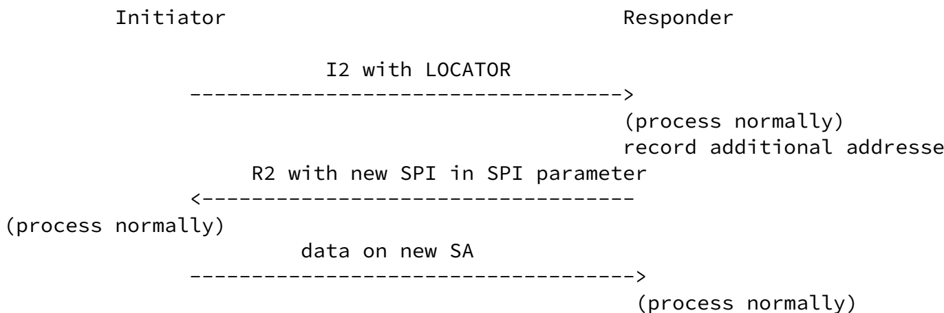
Figure 11: LOCATOR inclusion in I2
