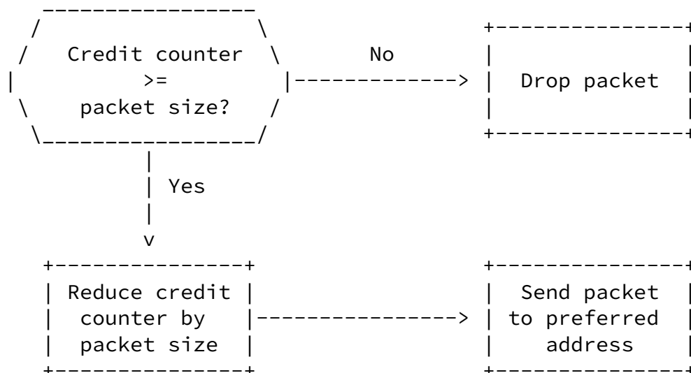
Figure 15: Sending Packets with Credit-Based Authorization
