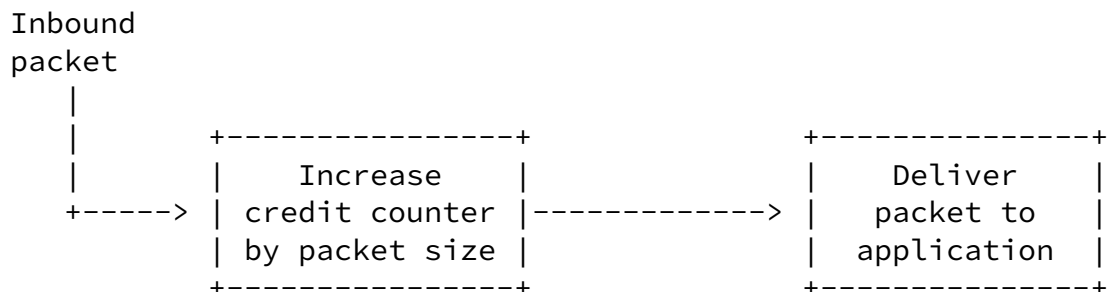
Figure 14: Receiving Packets with Credit-Based Authorization
