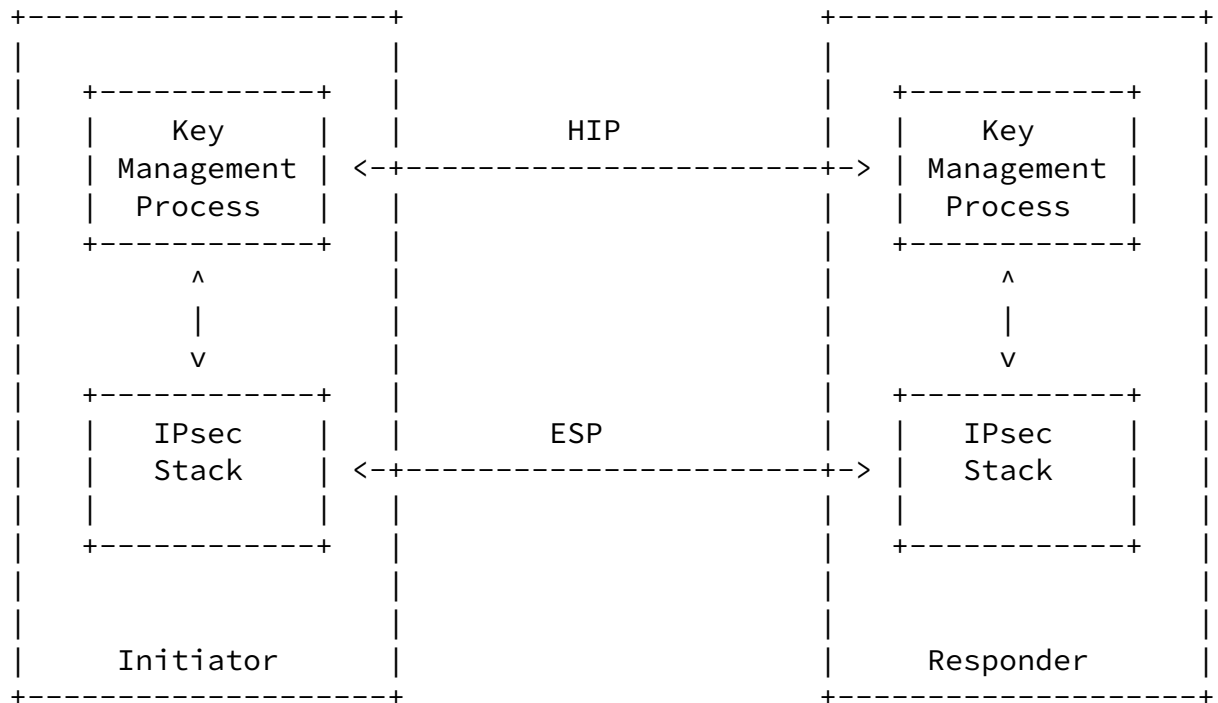
Figure 1: HIP deployment model
