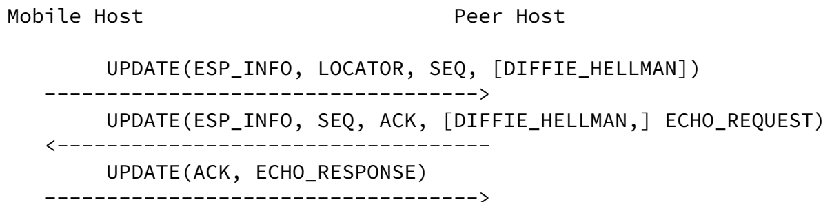
Figure 4: Readdress with mobile-initiated rekey
