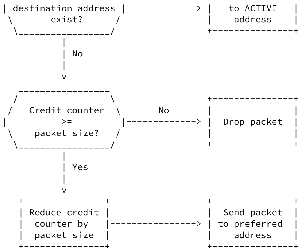
Figure 15: Sending Packets with Credit-Based Authorization
