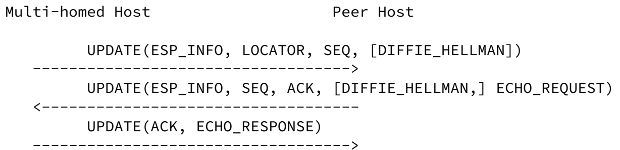
Figure 3: Basic Multihoming Scenario
