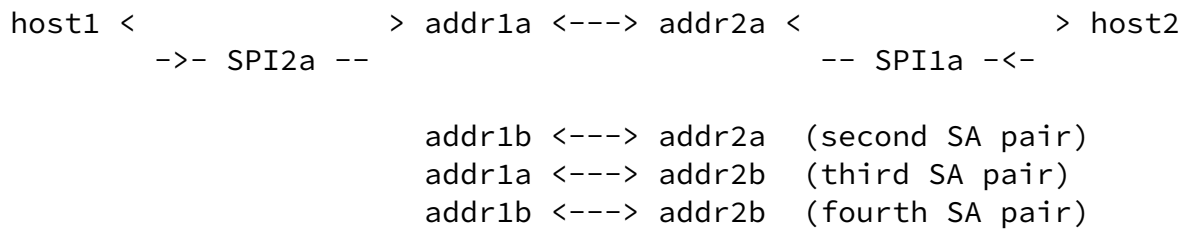
Figure 2: Dual Multihoming Case in Which Each Host Uses LOCATOR_SET to Add a Second Address
