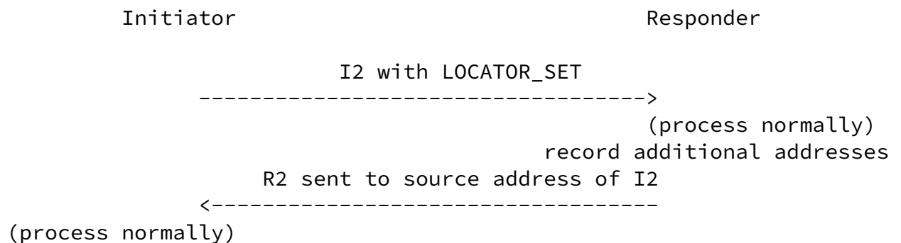
Figure 4: LOCATOR_SET Inclusion in I2
