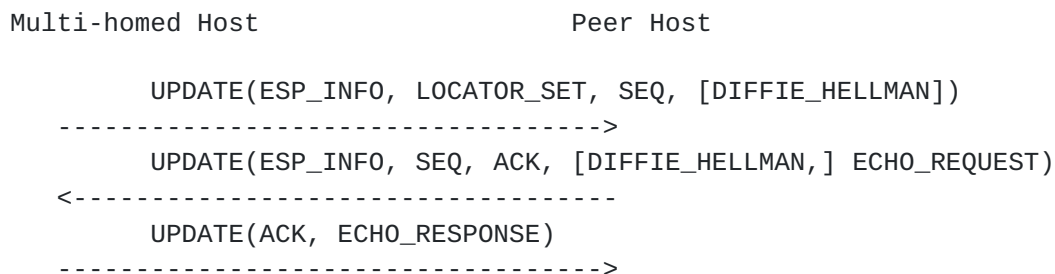
Figure 1: Basic Multihoming Scenario
