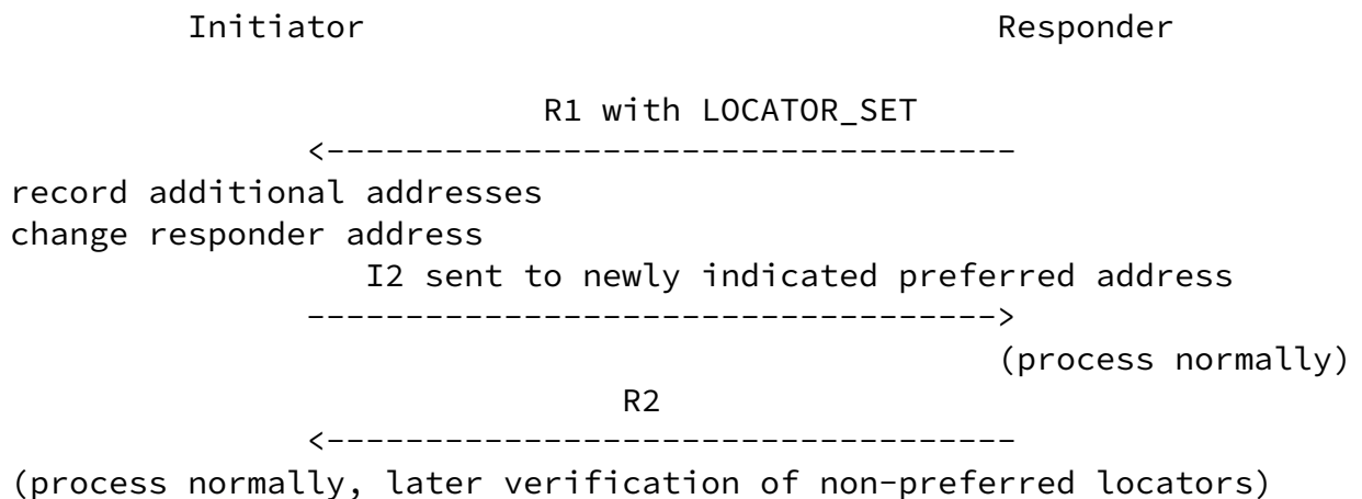
Figure 3: LOCATOR_SET Inclusion in R1
