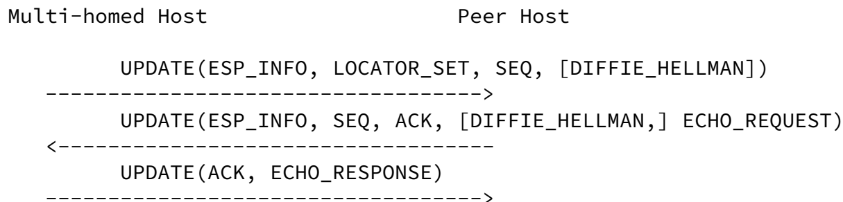
Figure 1: Basic Multihoming Scenario
