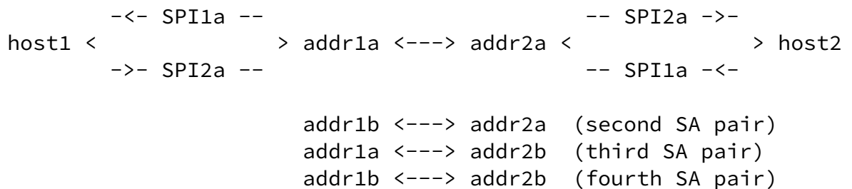
Figure 2: Dual Multihoming Case in Which Each Host Uses LOCATOR_SET to Add a Second Address
