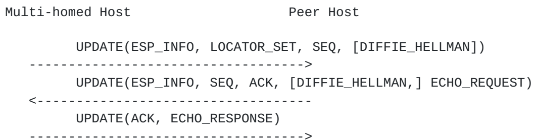
Figure 2: Host Multihoming for Load Balancing
