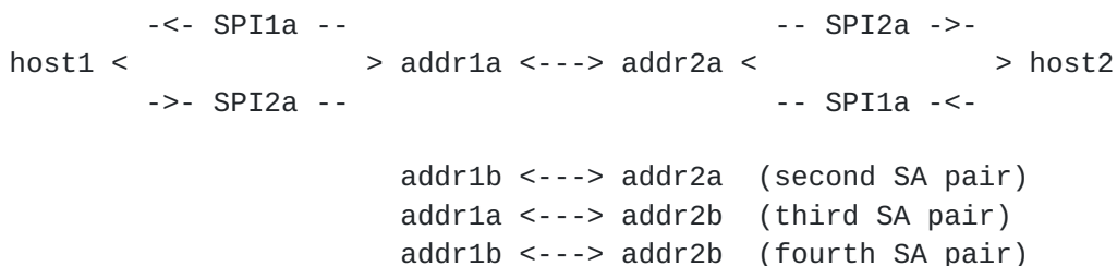
Figure 3: Dual Multihoming Case in Which Each Host Uses LOCATOR_SET to Add a Second Address
