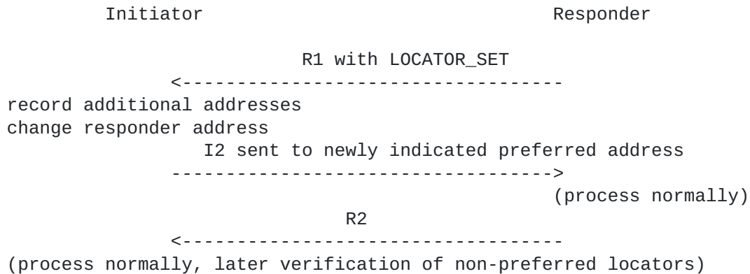
Figure 4: LOCATOR_SET Inclusion in R1
