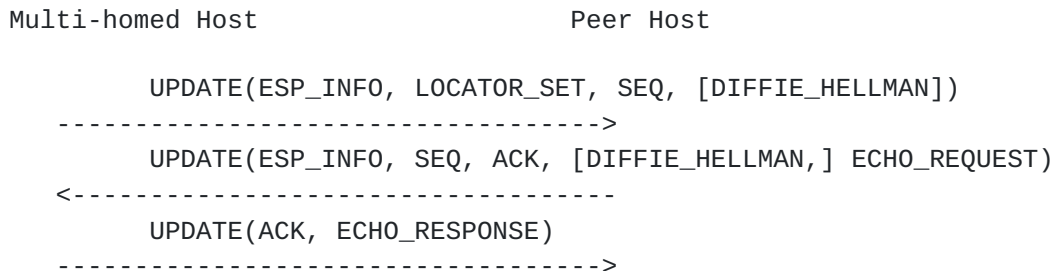
Figure 2: Host Multihoming for Load Balancing
