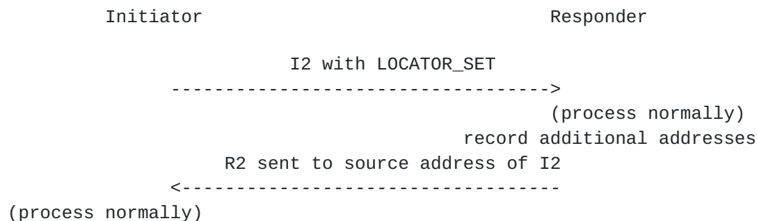
Figure 5: LOCATOR_SET Inclusion in I2
