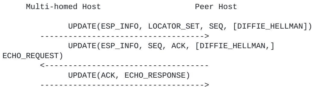
Figure 2: Host Multihoming for Load Balancing
