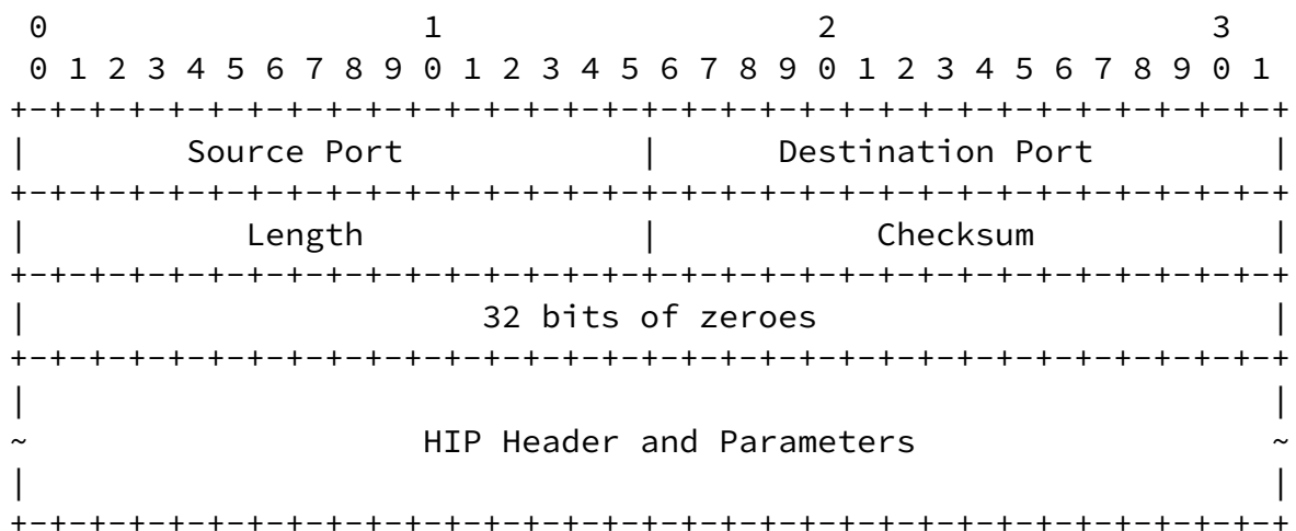
Figure 5: Format of UDP-encapsulated HIP Control Packets
