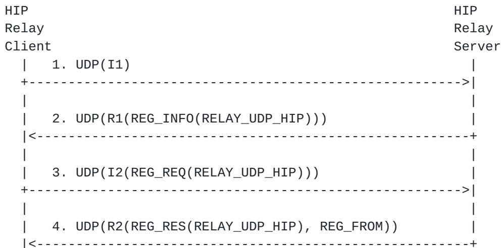
Figure 2: Example Registration with a HIP Relay
