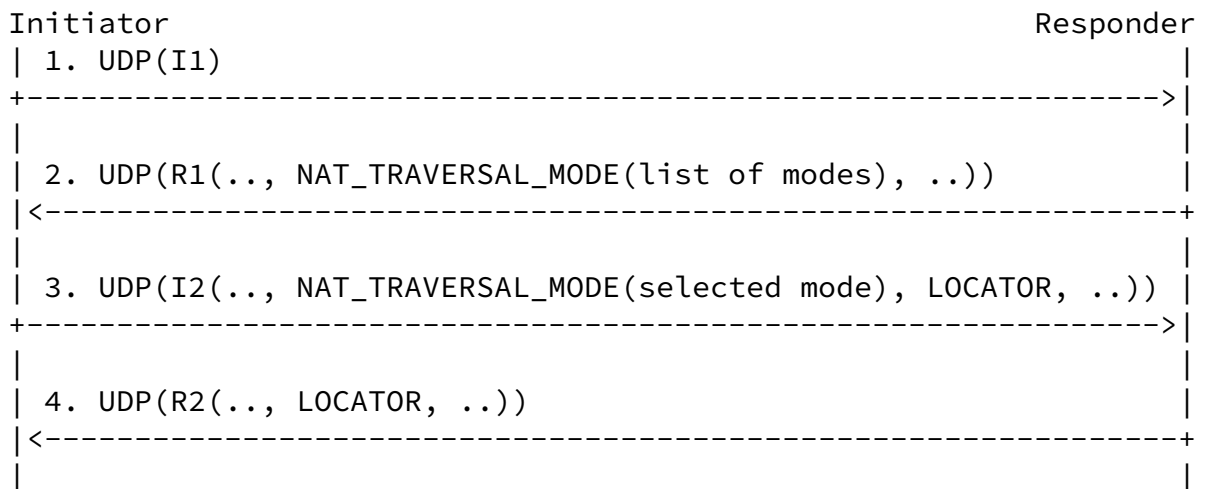
Figure 3: Negotiation of NAT Traversal Mode
