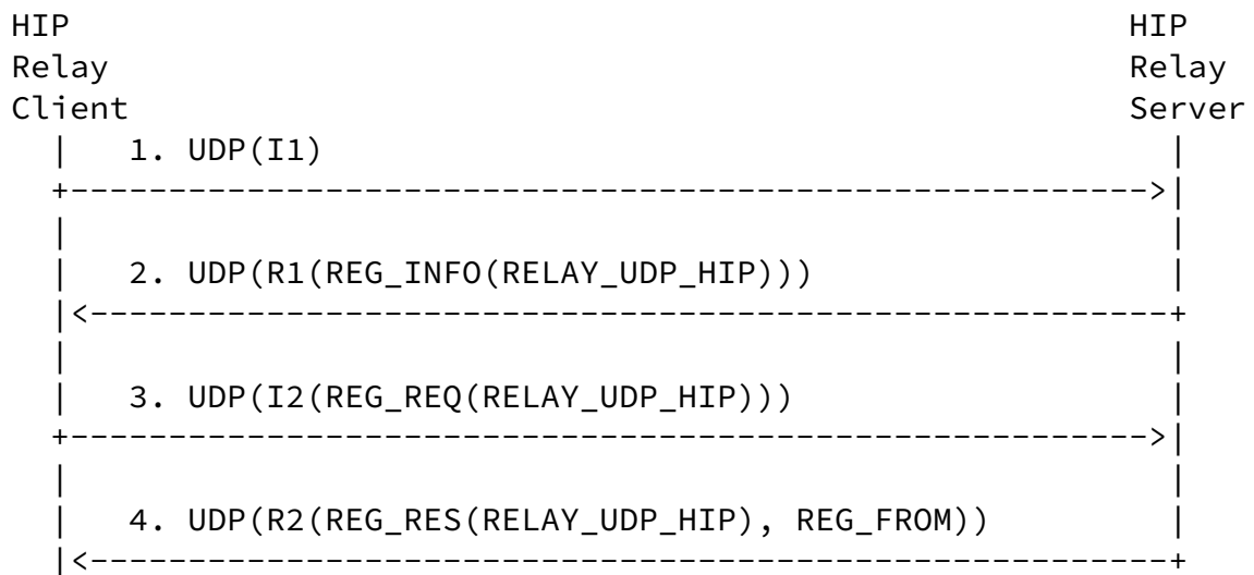
Figure 2: Example Registration with a HIP Relay
