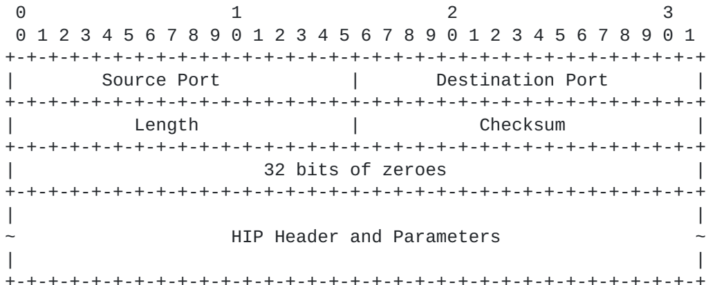
Figure 7: Format of UDP-Encapsulated HIP Control Packets
