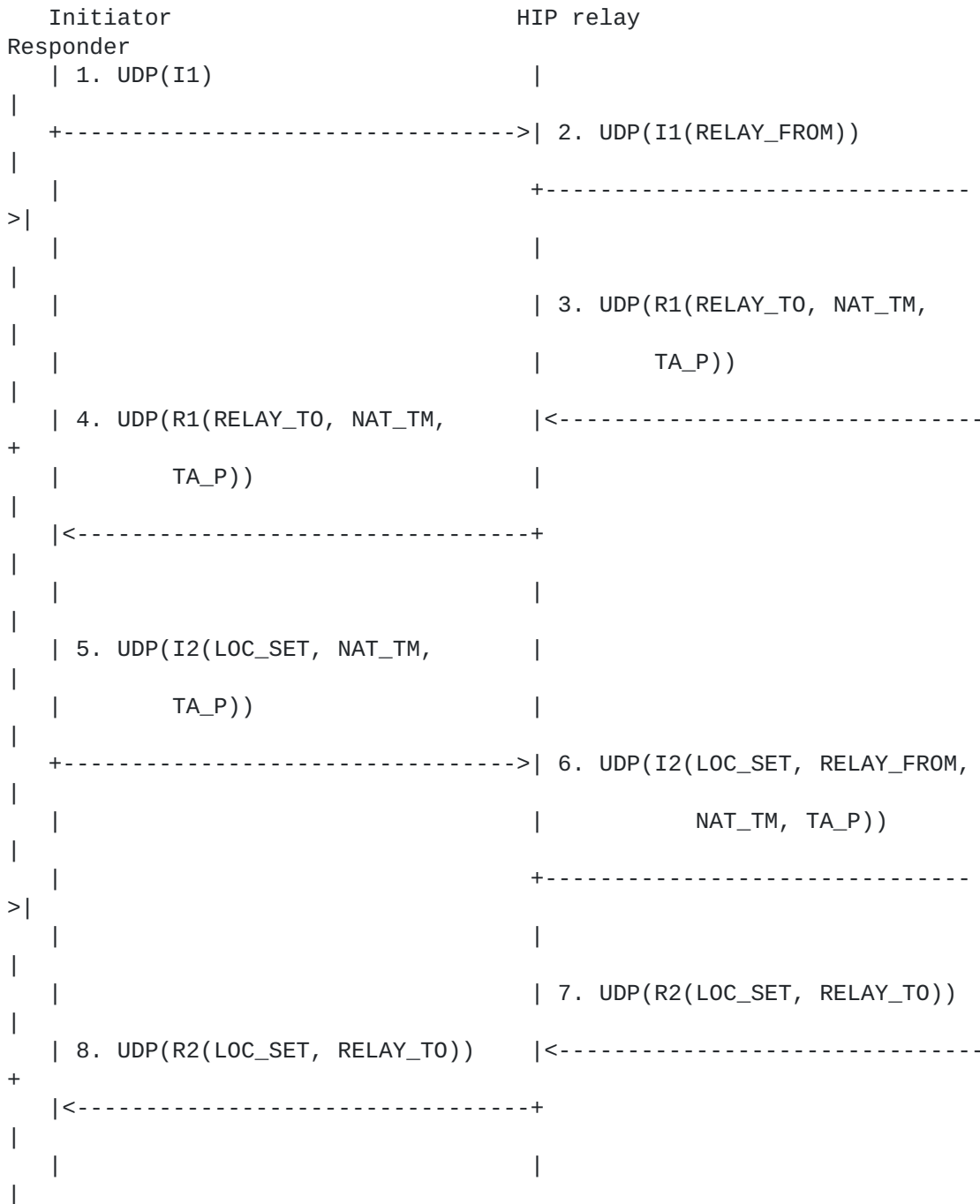
Figure 4: Base Exchange via a HIP Relay Server
