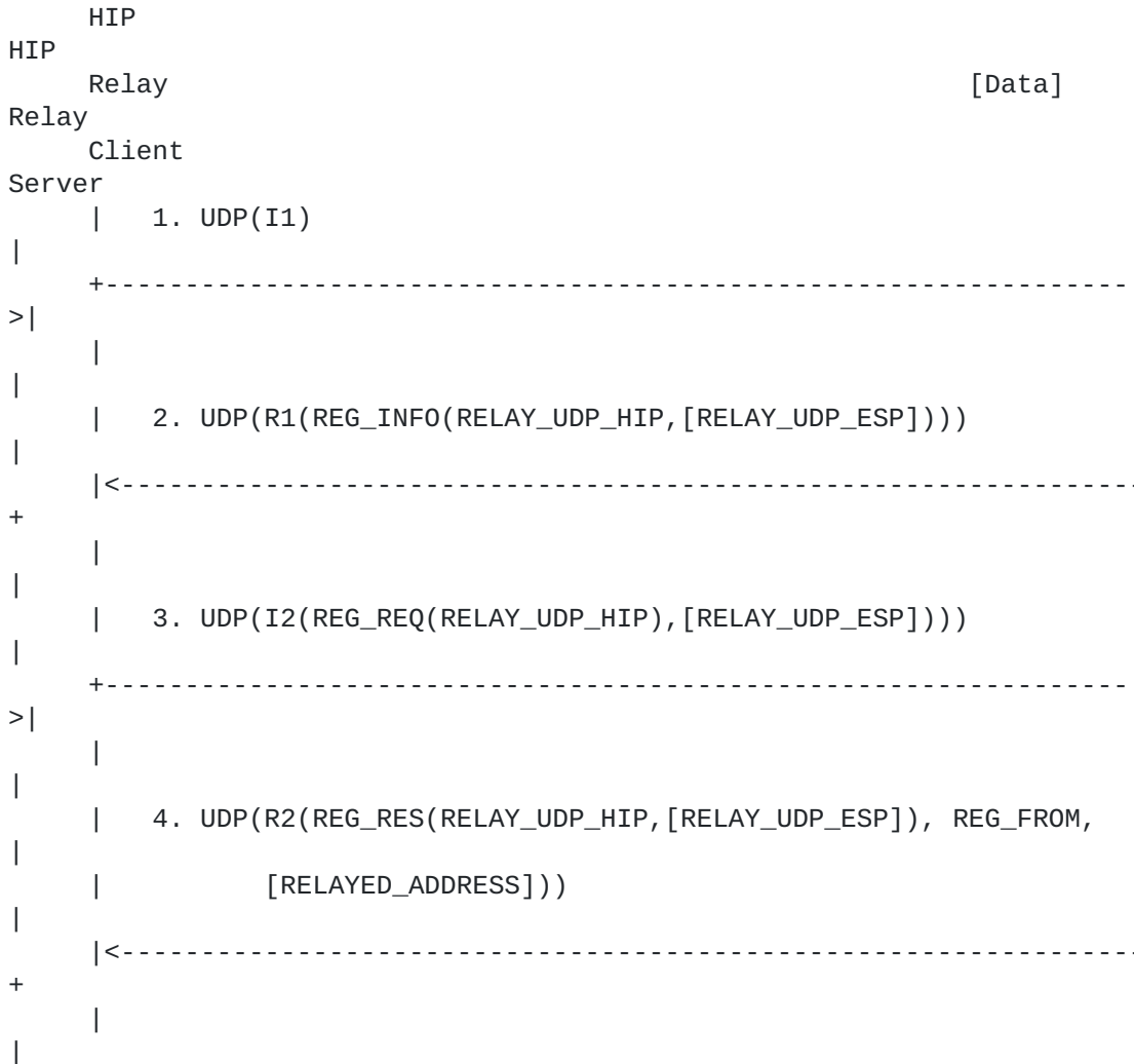
Figure 2: Example Registration with a HIP Relay
