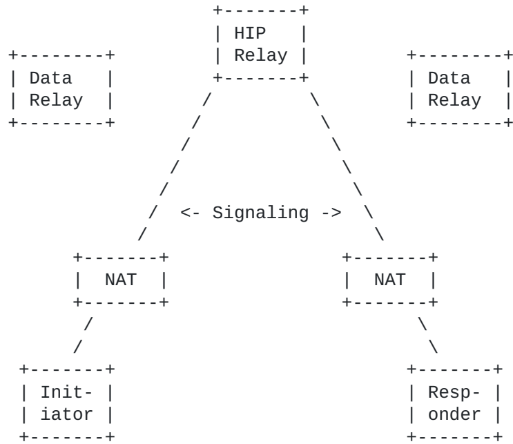
Figure 1: Example Network Configuration
