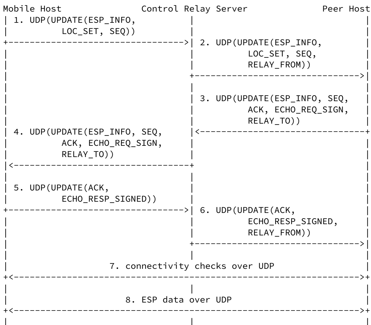
Figure 6: HIP UPDATE procedure
