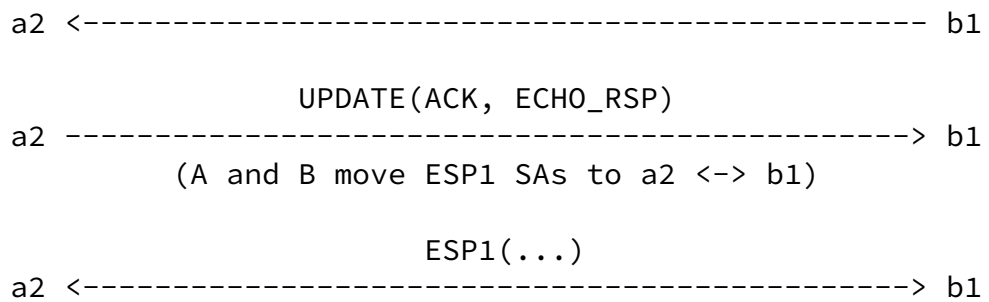
Figure 3: Break Before Make
